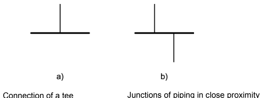
Figure 4 — Representation of connected pipes
