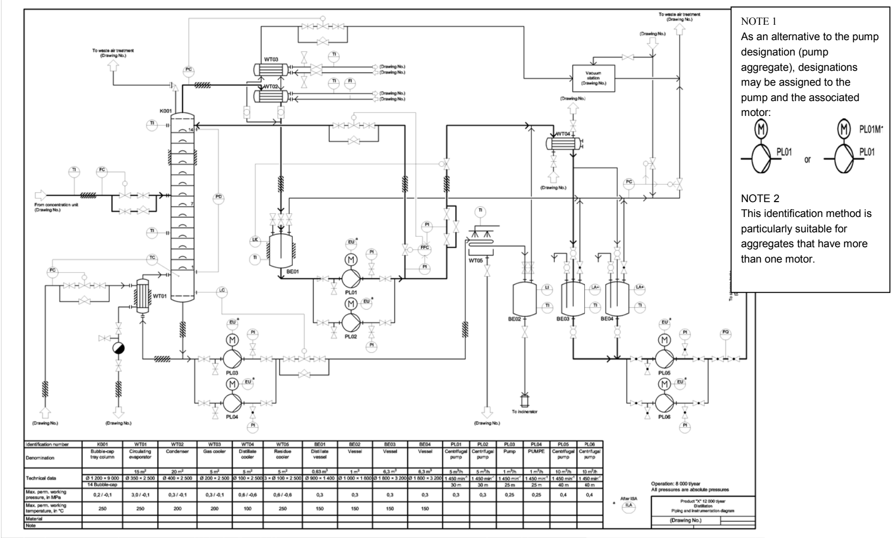
Figure A.6 — Piping and instrumentation diagram (P&ID) with basic information
