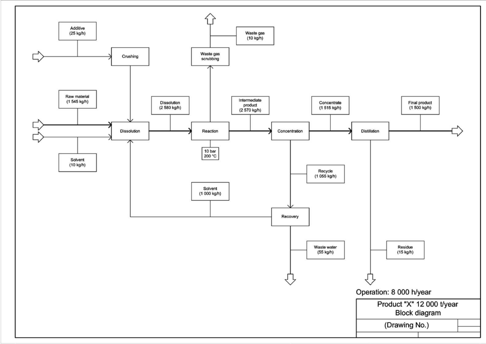
Figure A.2 — Block diagram with basic and additional information
