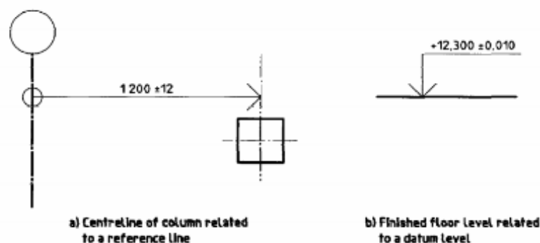
Figure 2 — Examples of limit deviations for position dimensions
