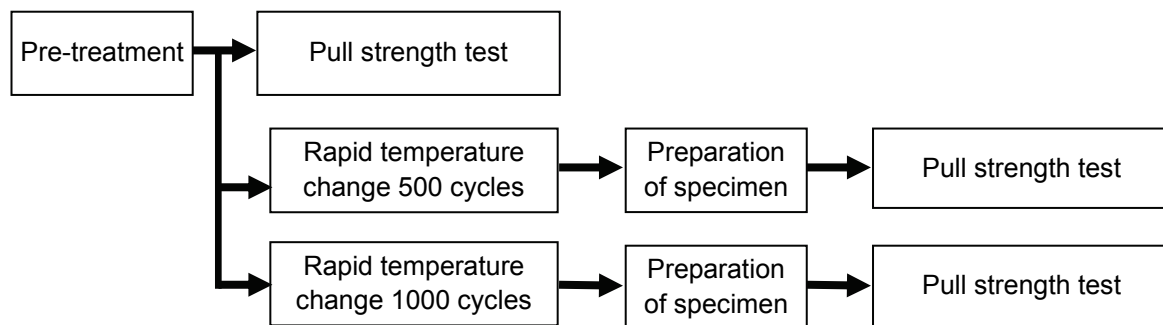
Figure 3 – Test procedure
