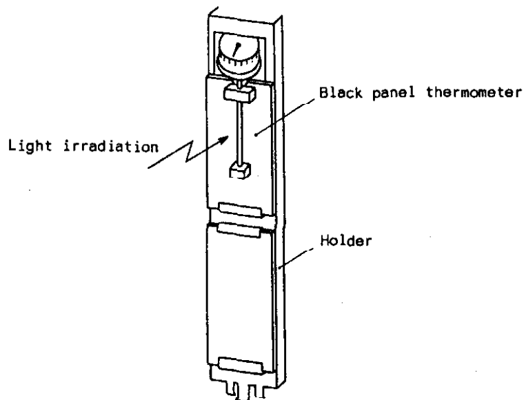
Informative Reference Fig. 1. Black Panel Thermometer
