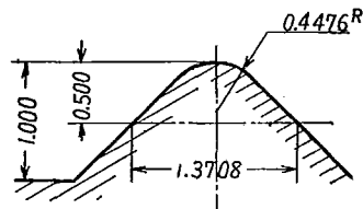
m = 1 hob tooth form
