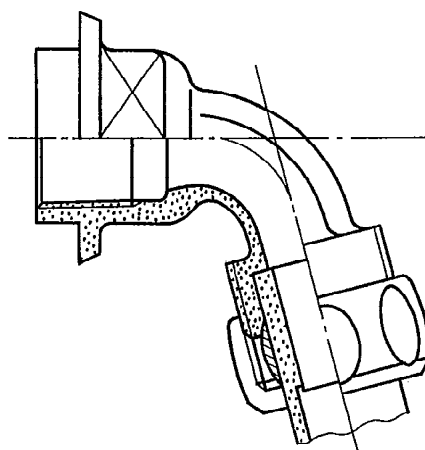
Faucet elbow
