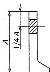
Bulb flat
