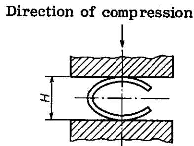
Fig. 2. Flattening Test (for C-shape Test Piece)
