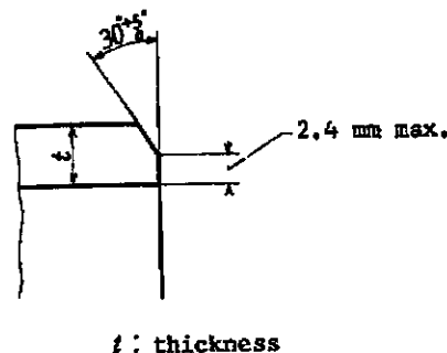
Fig. 1. Shape of Bevel End
