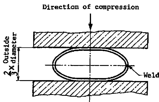
Fig. 2. Flattening Test
