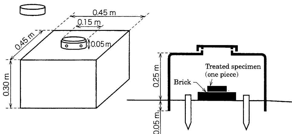
Figure 2 Box type container for field test
