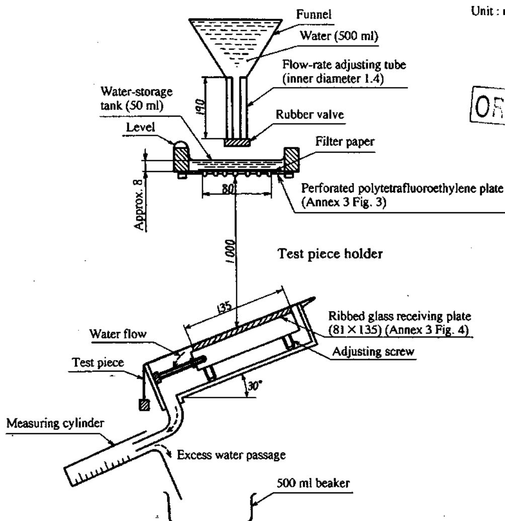
Annex 3 Fig. 2 Shower tester
