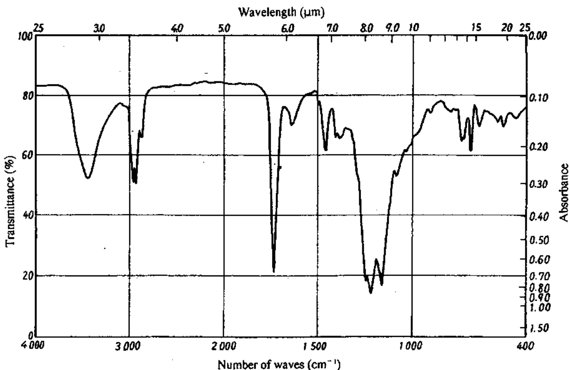
Annex 2 Fig. 12-1 Fluorine Part 1
