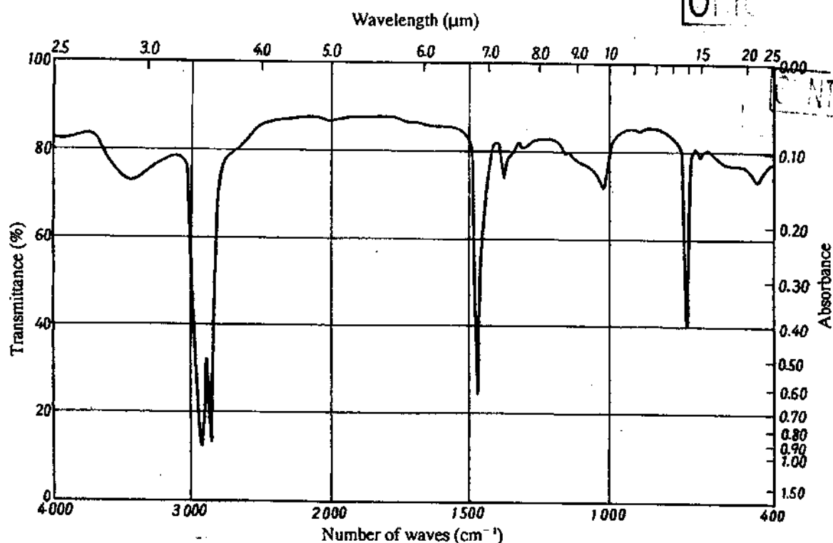
Annex 2 Fig. 4 Polyethylene
