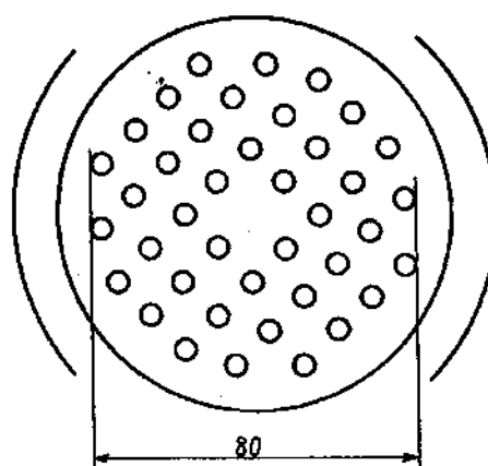
Annex 3 Fig. 2 Shower tester
