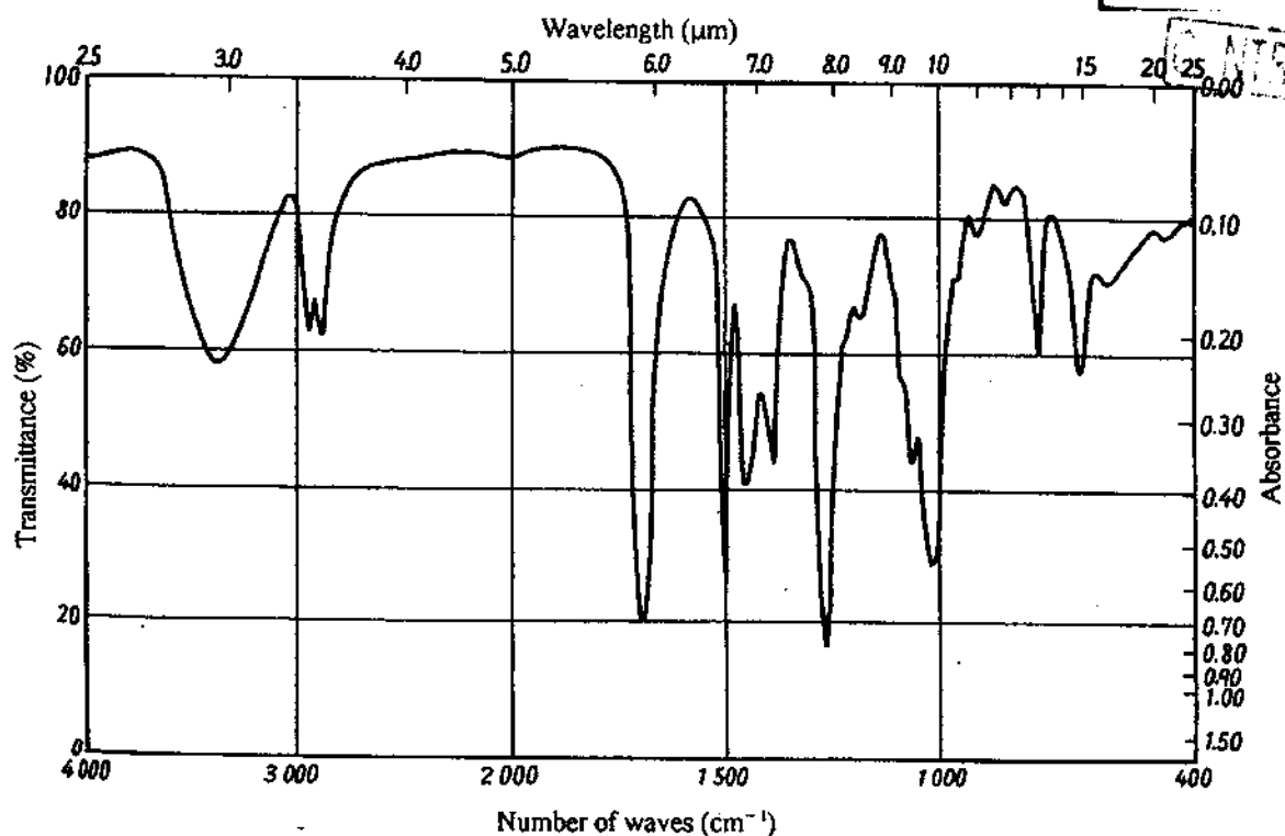
Annex 2 Fig. 8 Ethylene urea
