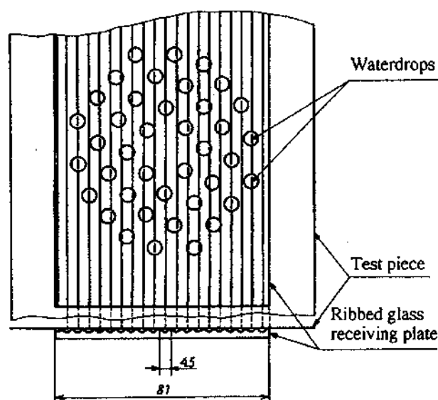
Annex 3 Fig. 4 Where shower waterdrops fall on the ribbed glass receiving plate
