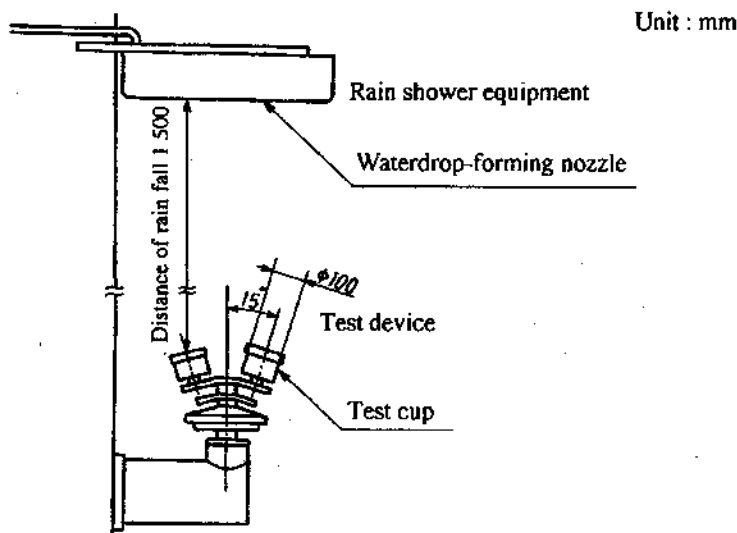
Fig. 6 Bundesmann rain-shower test apparatus
