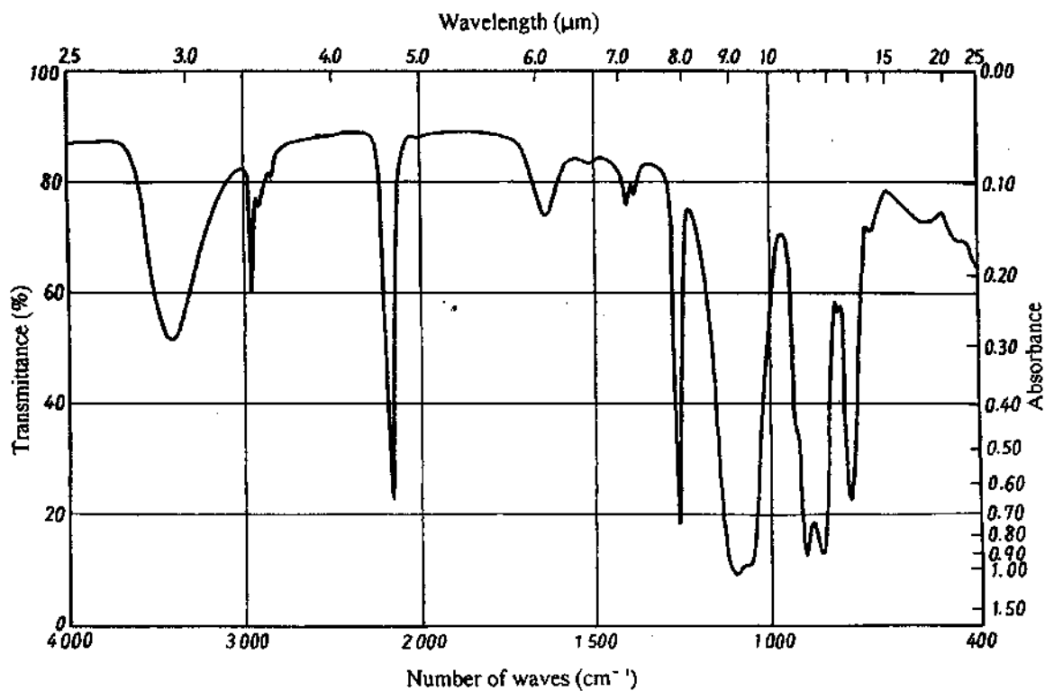
Annex 2 Fig. 11-3 Silicon Part 3
