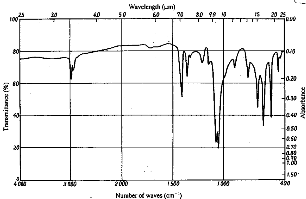
Annex 2 Fig. 2 Polyvinyliden chloride
