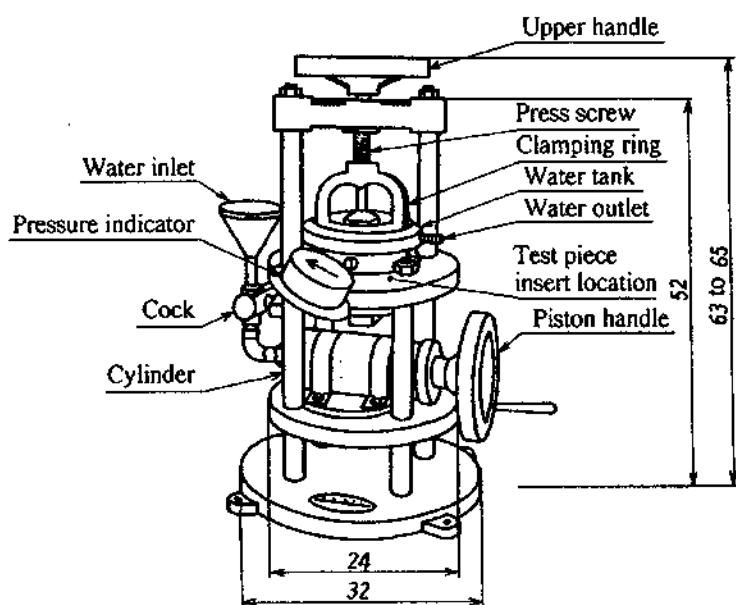
Fig. 3 Water penetration test apparatus (for high hydraulic pressure)
