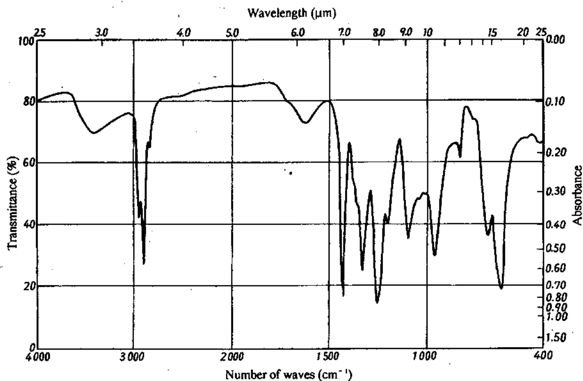
Annex 2 Fig. 3 Polyvinyl chloride
