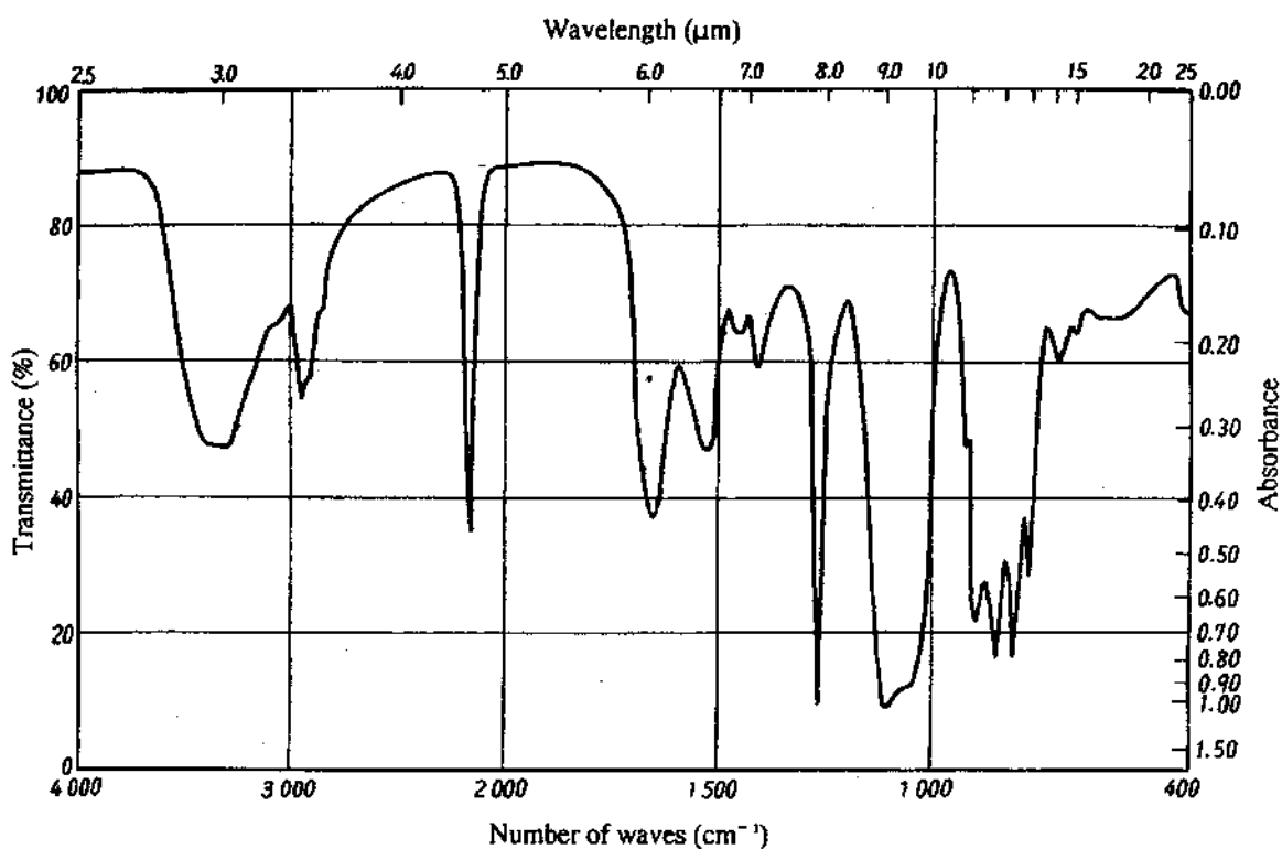
Annex 2 Fig. 11-1 Silicon Part 1
