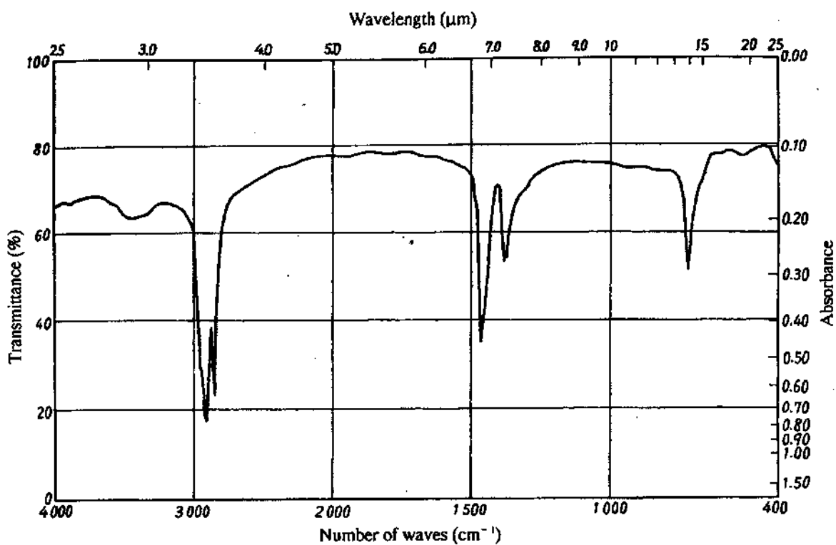
Annex 2 Fig. 7 Paraffin
