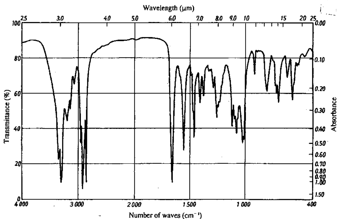
Annex 2 Fig. 10 Methylolamide
