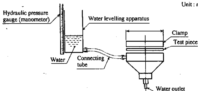
Fig. 2 Water penetration test apparatus (for low hydraulic pressure)
