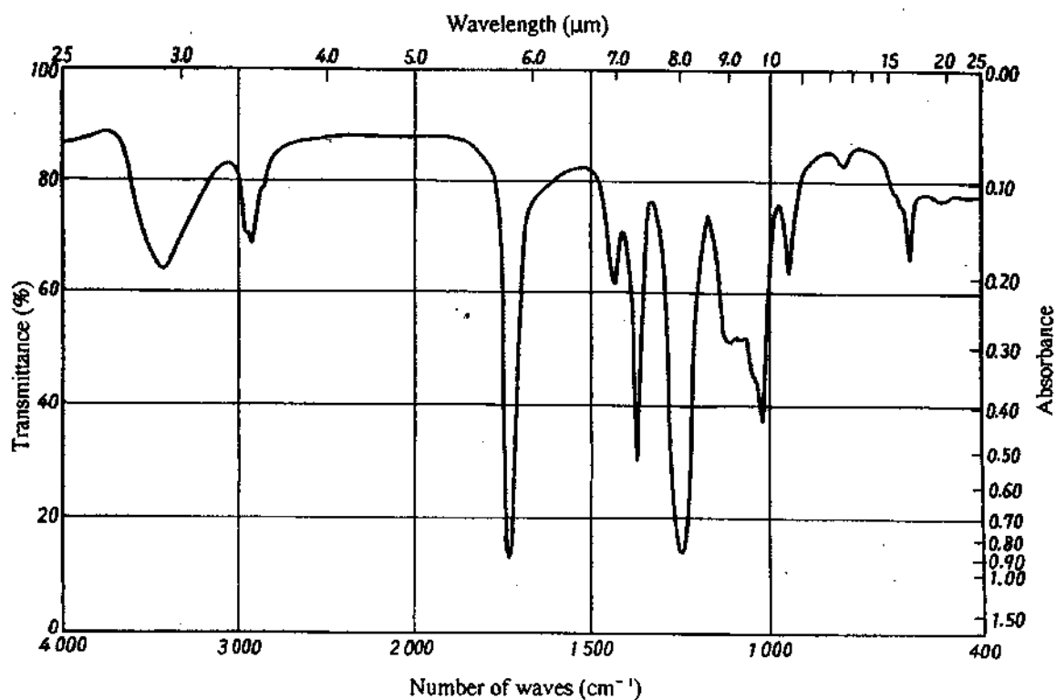
Annex 2 Fig. 5 Polyvinyl acetate
