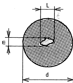
Figure E.1a) — Flaw smaller than the cross-section d of the useful ultrasonic beam
