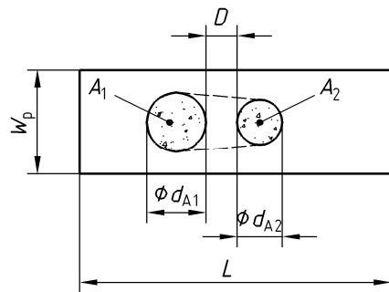
Figure C.1 — Clustered porosity, D > d_{A2}
