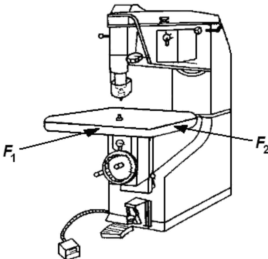
Figure B.1 — Stability test for displaceable machines
