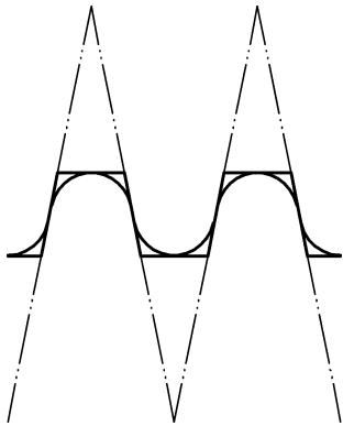
Figure B.3 — Idealisation of round shaped thread
