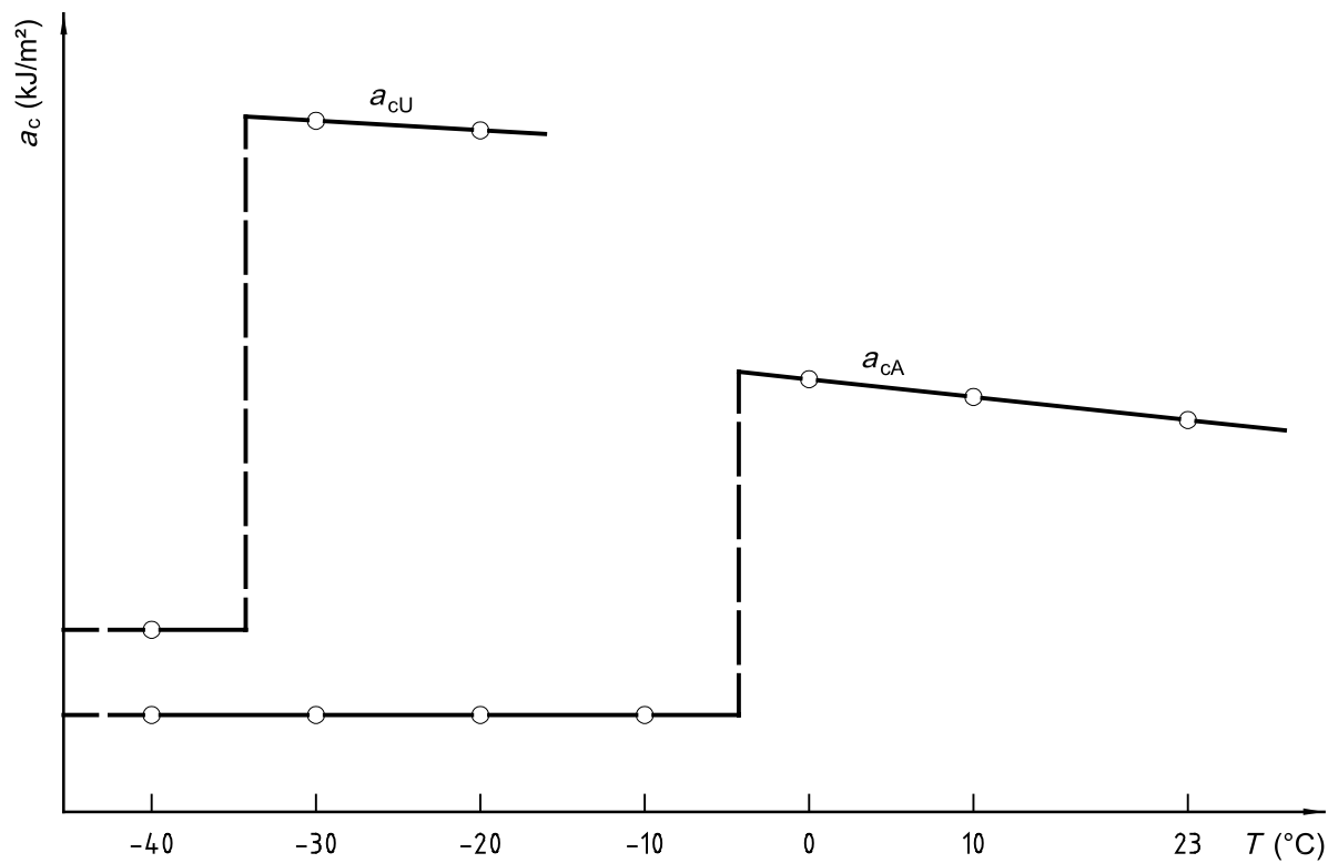
Figure 4 — Schematic diagram showing the variation of the Charpy impact strength a_c with temperature of notched and unnotched specimens
