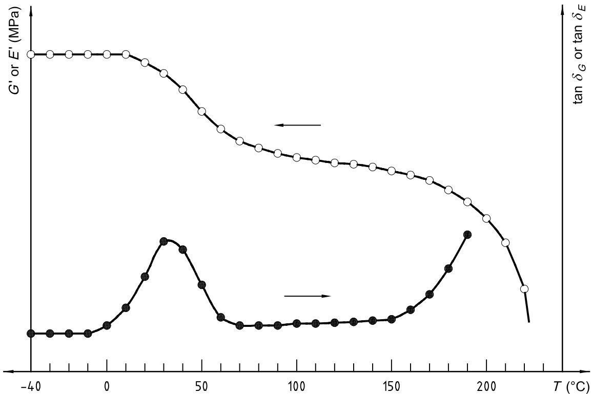
Figure 1 — Schematic diagram depicting the variation of the real part of the dynamic shear or tensile modulus, G' or E' respectively, and the damping factor of a semi-crystalline polymer with temperature T showing the glass-to-rubber relaxation region and the early stages of melting
