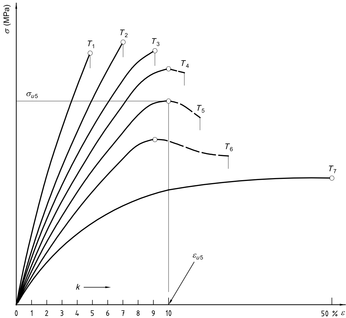
Figure 2 — Stress-strain curves at different temperatures T_i showing ultimate values of stress \sigma_{ui} and strain \epsilon_{ui} and identifying strains \epsilon_{ki} = \epsilon_{ui} \times k/10 at which values of stress are to be recorded
