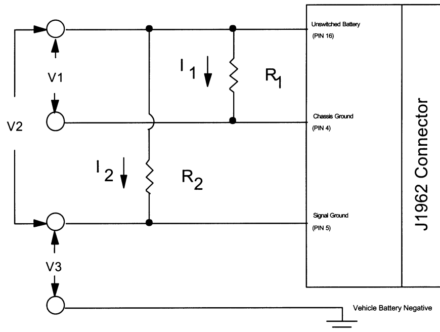
FIGURE B1—TEST SETUP FOR OBD-II SCAN TOOL POWER LOAD INTERFACE
