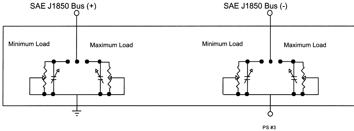
FIGURE 6—SAE J1850 NETWORK LOAD BOX
