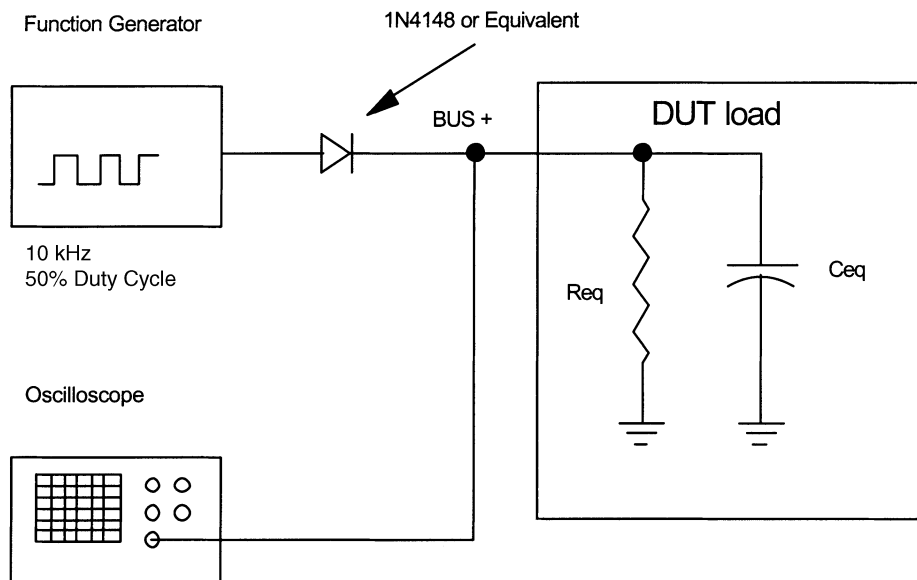
FIGURE C2—SETUP FOR BUS + CAPACITANCE MEASUREMENT
