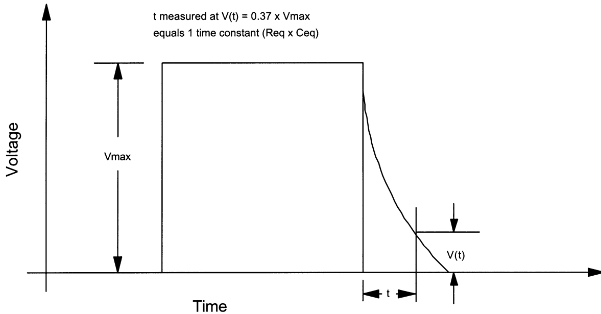
FIGURE C3—BUS + CAPACITANCE WAVEFORM
