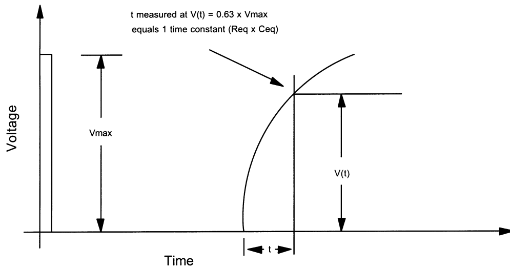
FIGURE C5—BUS - CAPACITANCE WAVEFORM
