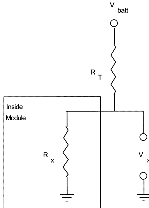
FIGURE C1—SETUP FOR BUS + RESISTANCE MEASUREMENT
