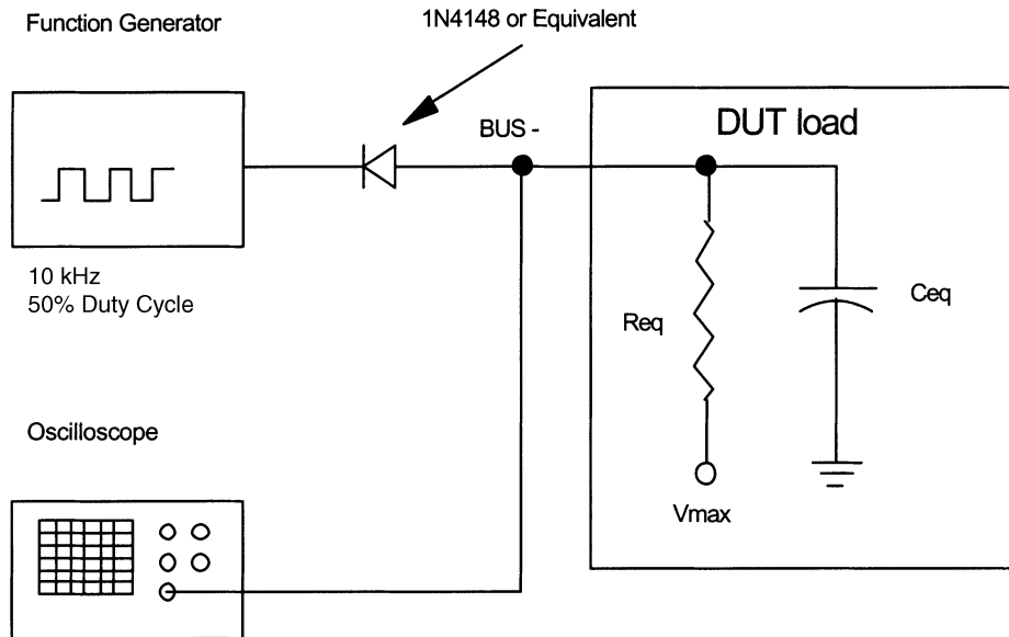
FIGURE C4—SETUP FOR BUS - CAPACITANCE MEASUREMENT
