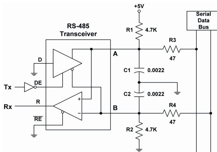
FIGURE A1—SERIAL DATA BUS STANDARD NODE DIAGRAM
