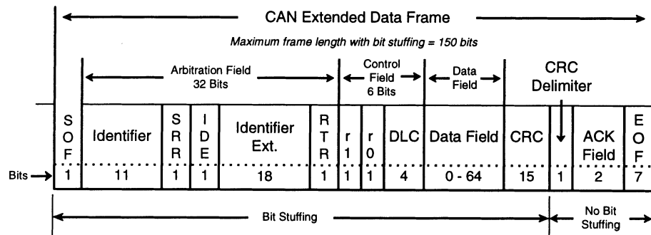
FIGURE 1—CAN DATA FRAMES
