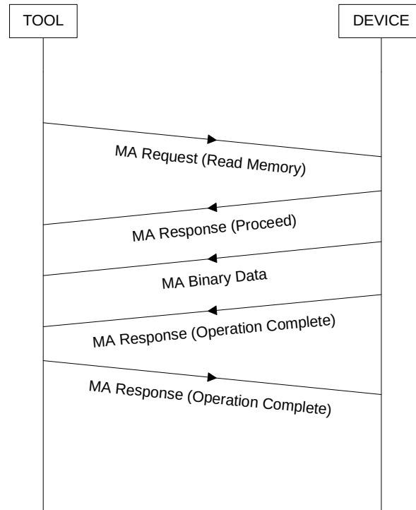
FIGURE E.2 EXAMPLE: MESSAGE SEQUENCE TO ACCOMPLISH MEMORY READ OPERATION WITHOUT SECURITY
