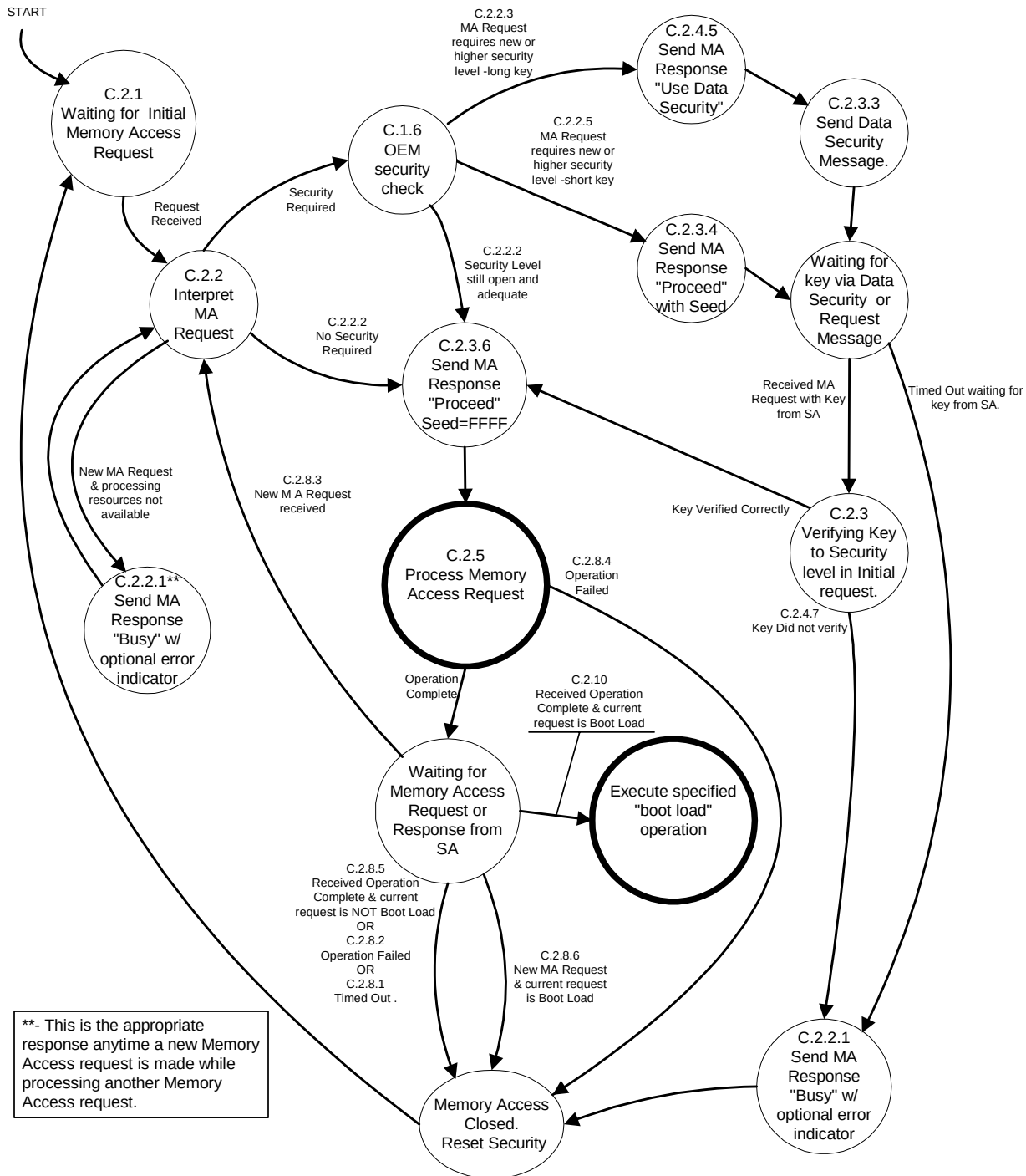
: C.1 MEMORY ACCESS STATE TRANSITION DIAGRAM
