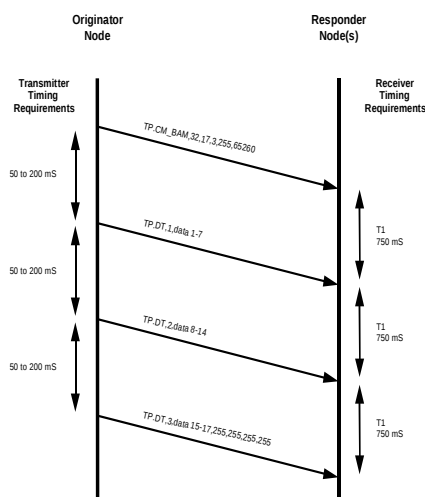
FIGURE C3 BROADCAST DATA TRANSFER
