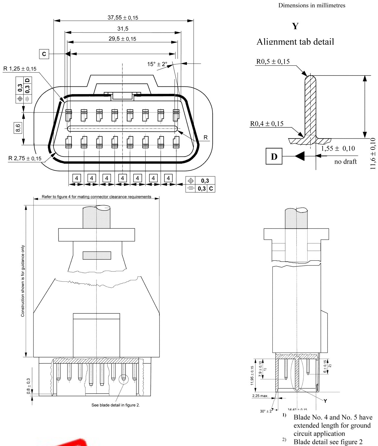
A2—EXTERNAL TEST EQUIPMENT CONNECTOR TYPE A
