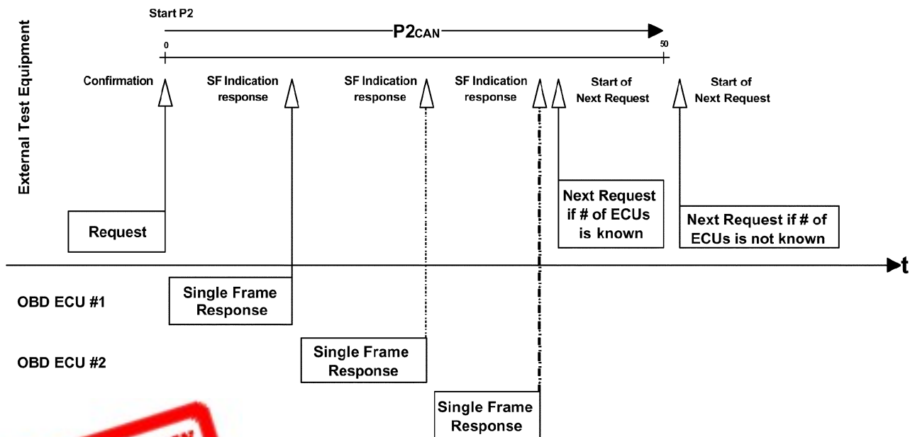
FIGURE 3—ISO 15765-4 APPLICATION TIMING PARAMETER OVERVIEW (SINGLE FRAME RESPONSE MESSAGES) OVERVIEW
