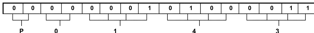
FIGURE 12—DIAGNOSTIC TROUBLE CODE ENCODING EXAMPLE DTC P0143
