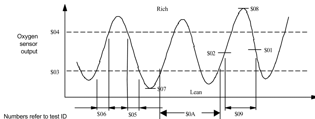
JRE 15—STANDARDIZED TEST ID VALUE EXAMPLE
