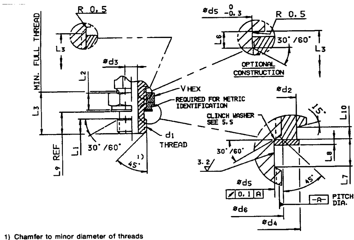
FIGURE 1A—ADJUSTABLE SAE J2244/2 HEAVY-DUTY (S SERIES) STUD END DETAIL
