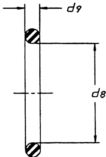
FIGURE 2—O-RING DETAIL
