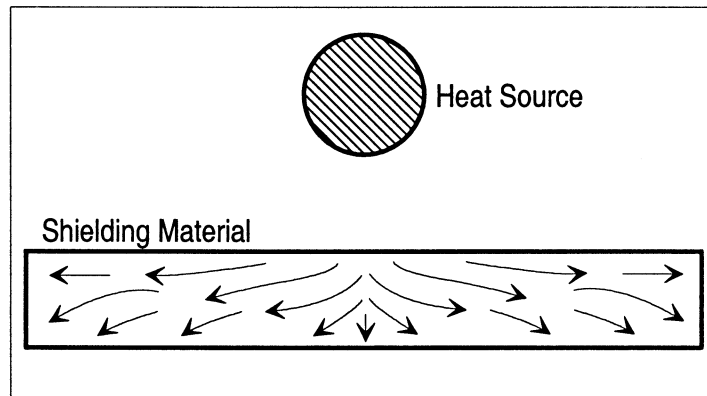
FIGURE 1—MULTI-DIMENSIONAL HEAT FLOW THROUGH SHIELDING MATERIAL WITH CENTRAL HEAT SOURCE
