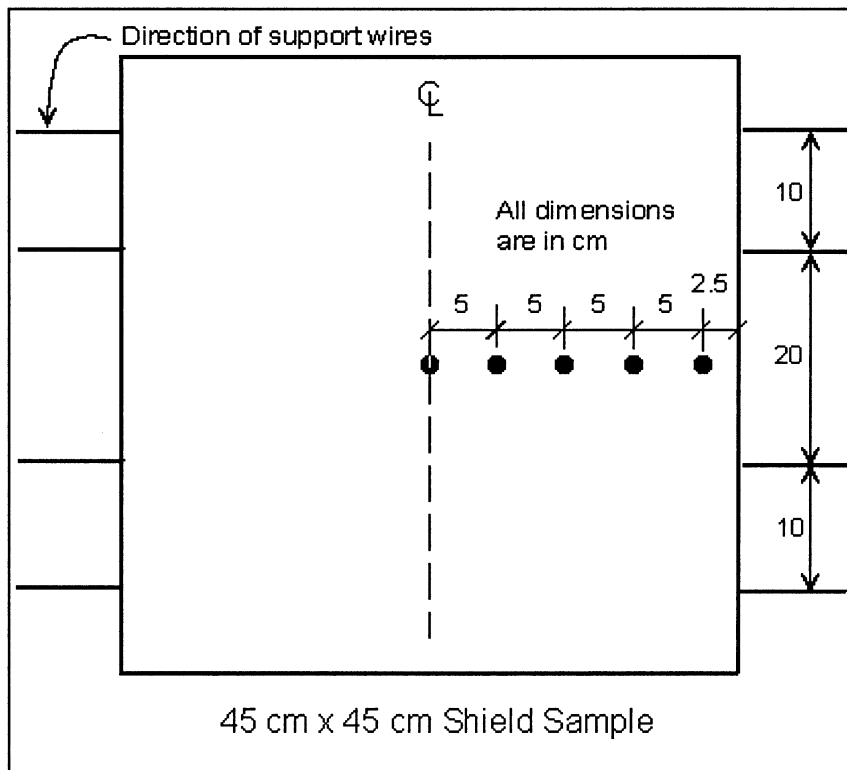
FIGURE 3—THERMOCOUPLE ARRANGEMENT ON 45 cm SAMPLE
