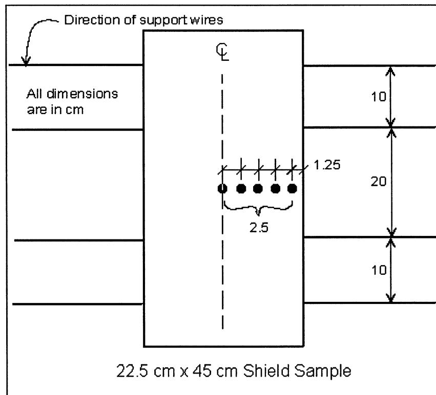
FIGURE 4—THERMOCOUPLE ARRANGEMENT ON 22.5 cm SAMPLE
