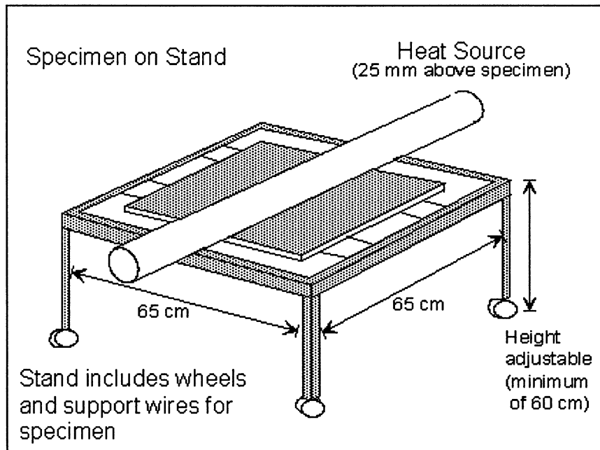
FIGURE 2—MAIN COMPONENTS OF EXPERIMENTAL SETUP
