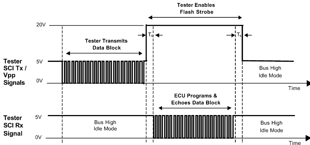
FIGURE 14—TESTER MULTIPLEXING OF THE SCI TX AND VPP FLASH STROBE SIGNALS FOR A SINGLE DATA BLOCK TRANSFER EVENT
