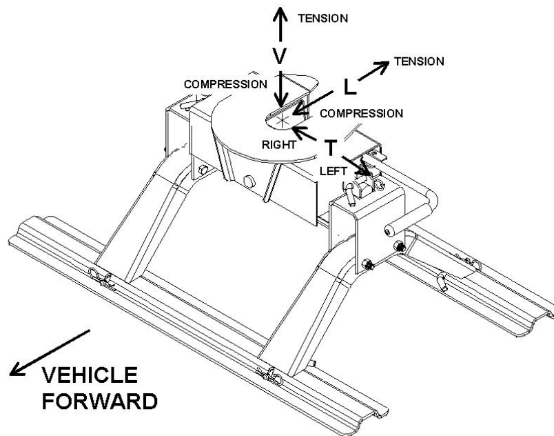
FIGURE 3—FIFTH WHEEL HITCH AND LOAD DIRECTION
