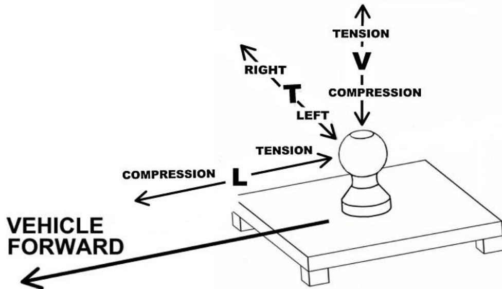
FIGURE 4—GOOSENECK HITCH AND LOAD DIRECTION
