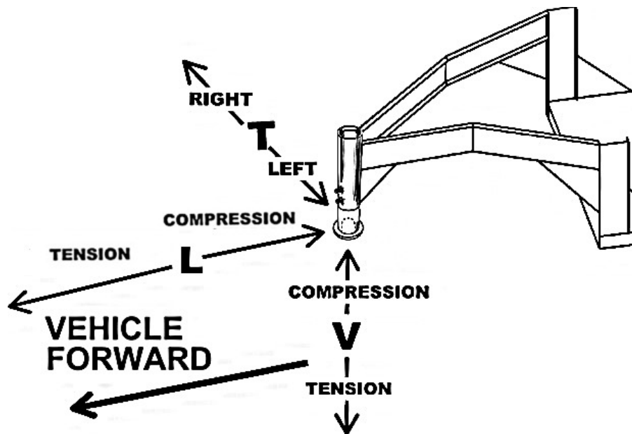
FIGURE 5—GOOSENECK STEM / TRAILER AND LOAD DIRECTION
