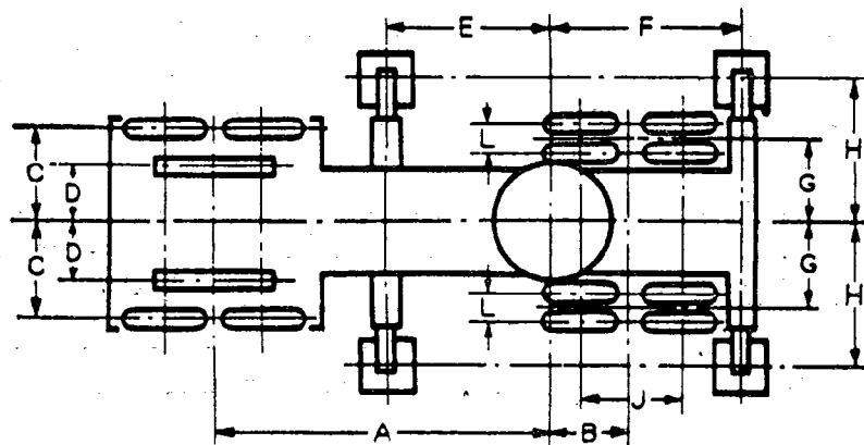
6 X 4 TRUCK
