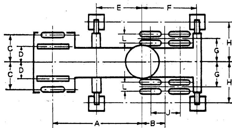
6 X 4 TRUCK
