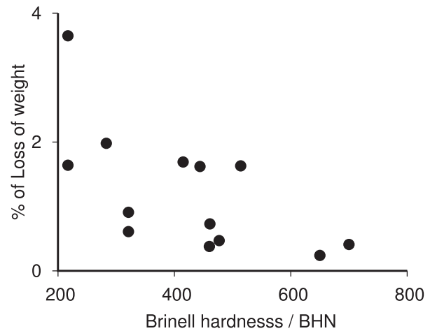
Figure 5. Data for field performance of wear resistance steel tools in ceramic industry. Data from [52].
