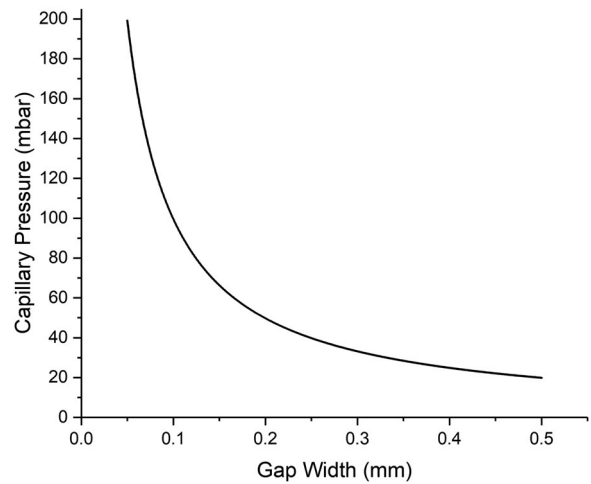
Figure 4. Plot illustrating the trend in capillary pressure with gap width, calculated using the Young-Laplace equation, taking \gamma (pure silver at T_m ) = 0.914 \text{ Nm}^{-2} and \theta = 57^\circ
