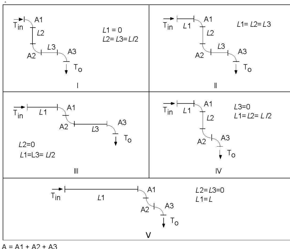
Figure D.1—Conduit layout—BendCorr factor
