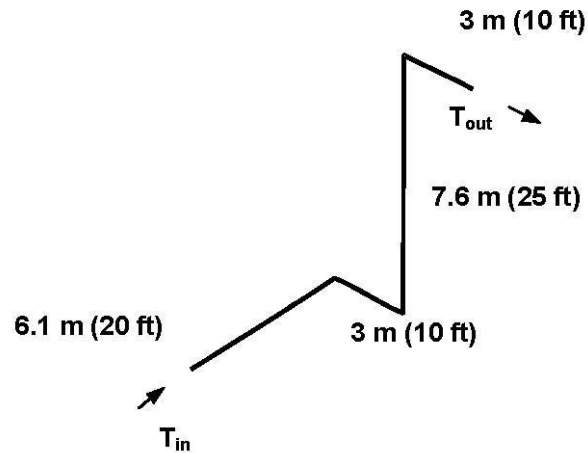
Figure B.3—Isometric of conduit layout—Example #3
