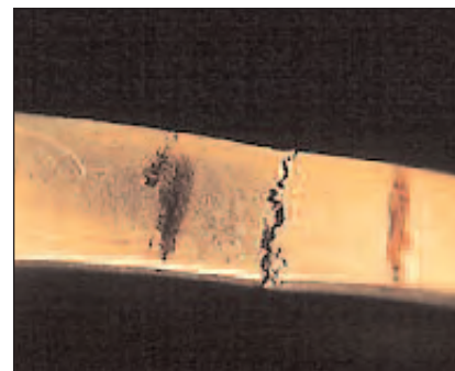
Fig. 19.1 A broken shank of an 18ct yellow gold ring
