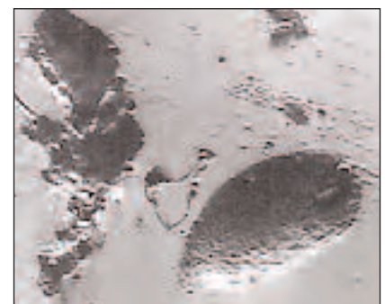
Fig. 14.2 Surface porosity on a 14ct yellow gold casting
