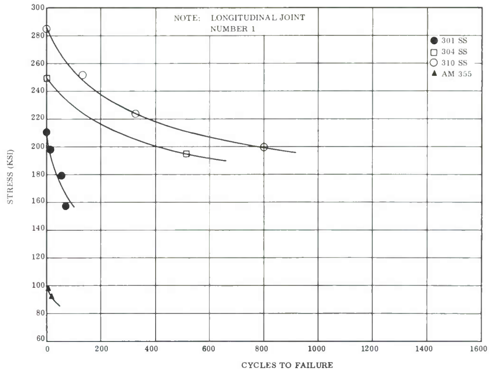
Figure 80. S-N Curve - Stainless Steels at -423°F (Longitudinal - Joint No. 1)
