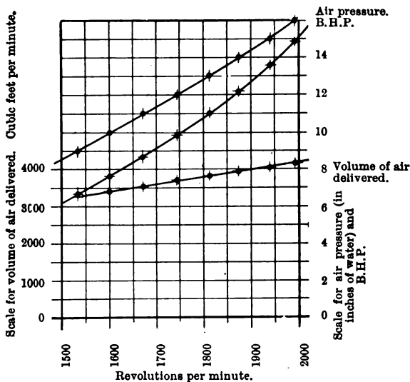
FIG. 23.—Results of trials of a 28 in. Heenan cupola fan.
