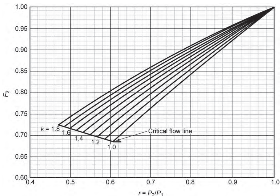
Figure 35—Values for F_2 for Subcritical Flow
