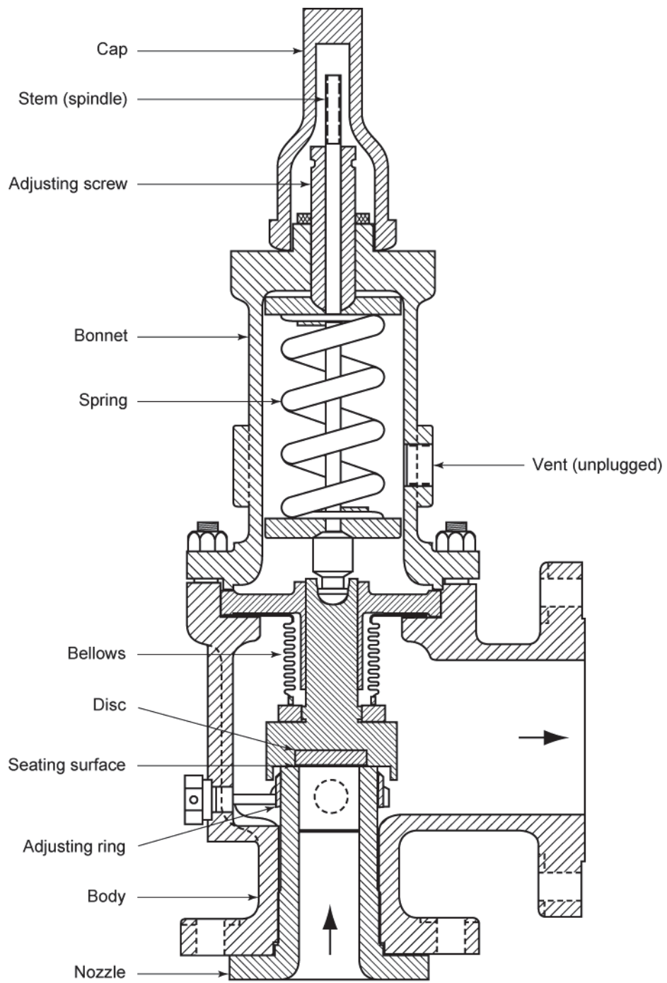
Figure 2—Balanced-bellows PRV
