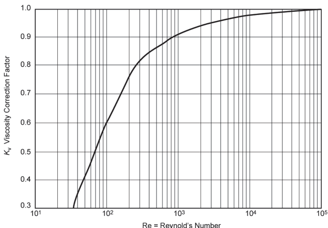
Figure 37—Capacity Correction Factor, K_v , Due to Viscosity
