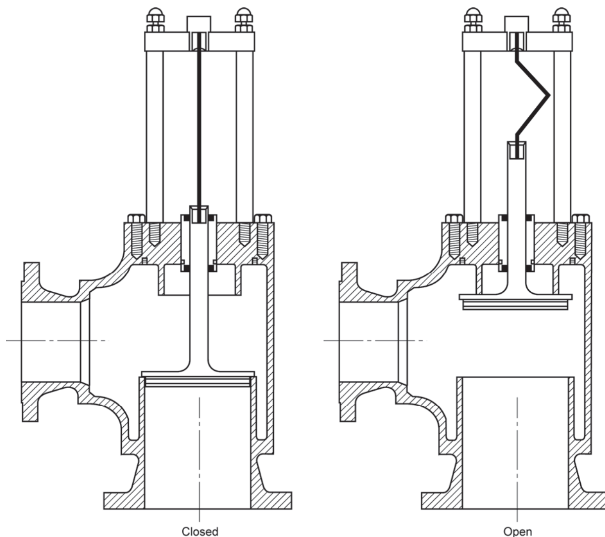
Figure 29—Buckling Pin Valve
