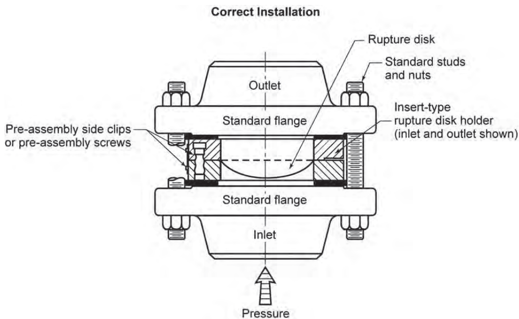
Figure 24—Reverse-acting Scored Rupture Disk
