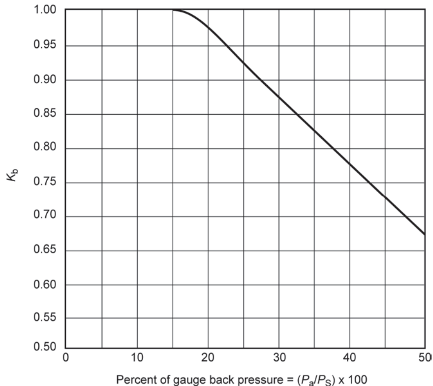
Figure C.3—Backpressure Correction Factor, K_b , for Balanced-bellows PRVs (Liquids)
