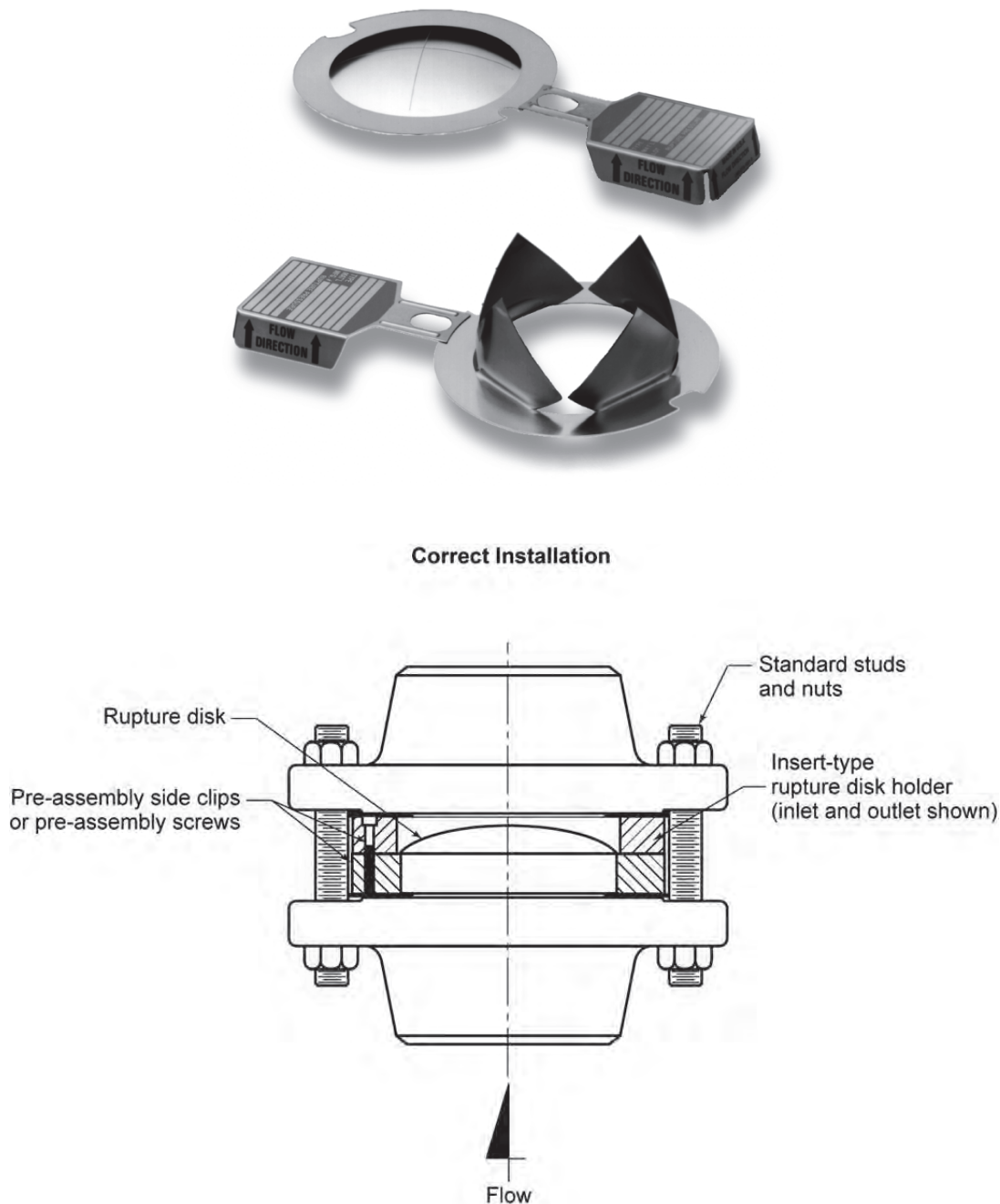
Figure 21—Forward-acting Scored Rupture Disk
