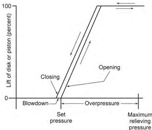
Figure 17—Typical Relationship Between Lift of Disk or Piston and Vessel Pressure in a Modulating-action Pilot-operated PRV
