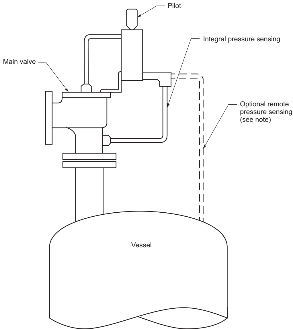
Figure 9—Typical Pilot-Operated Pressure-relief Valve Installation
