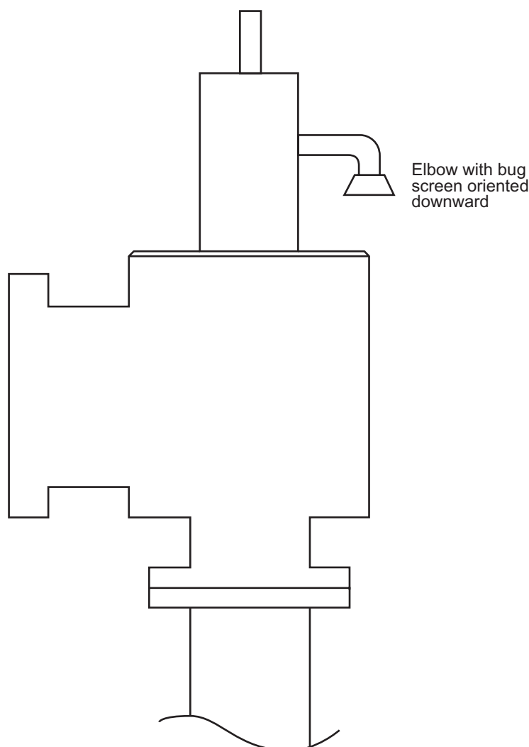
Figure 20—Bonnet Vent for Bellows Valves with Vent Located at the PRV
