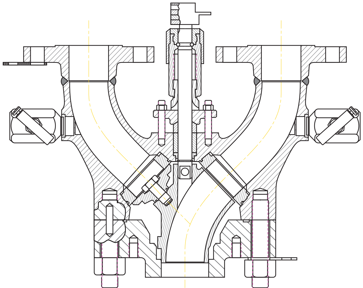
Figure 15—Three-Way Changeover Valve—Rotor Type
