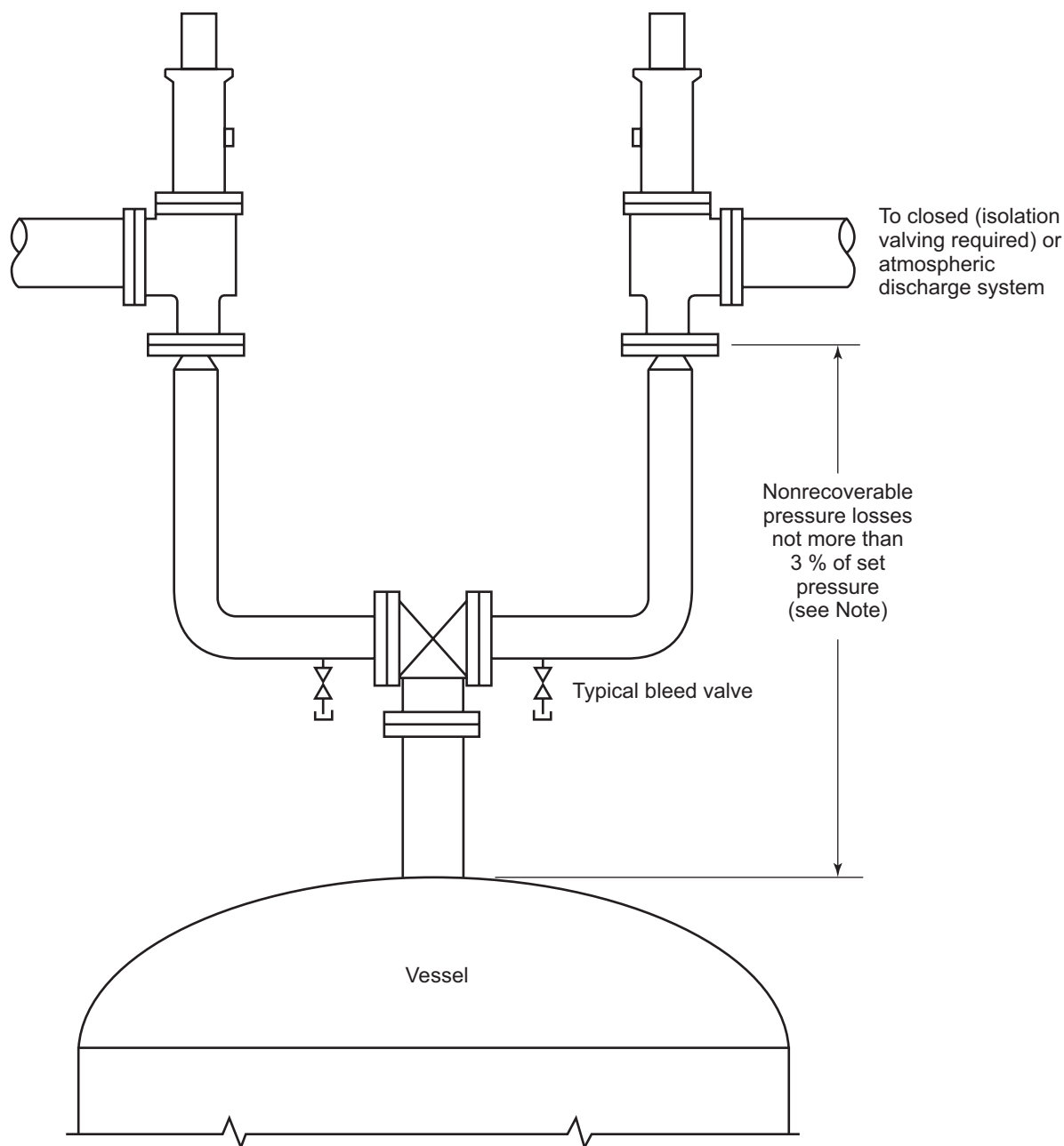
Figure 11—Typical PRD Installation for 100 % Spare Relieving Capacity
