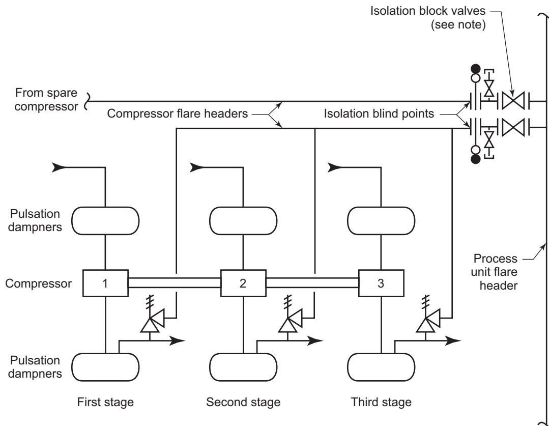
Figure 18—Typical Isolation Block Valves for Spare Compressor
