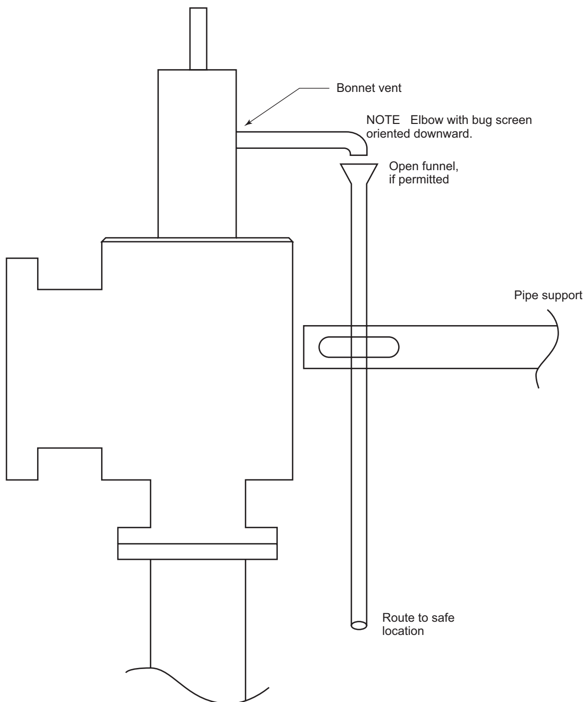
Figure 22—Bonnet Vent for Bellows Valves Handling Liquids Where a Leak Needs to Be Routed Away from the PRV
