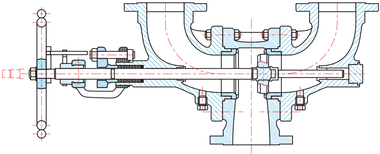
Figure 14—Three-Way Changeover Valve—Shuttle Type
