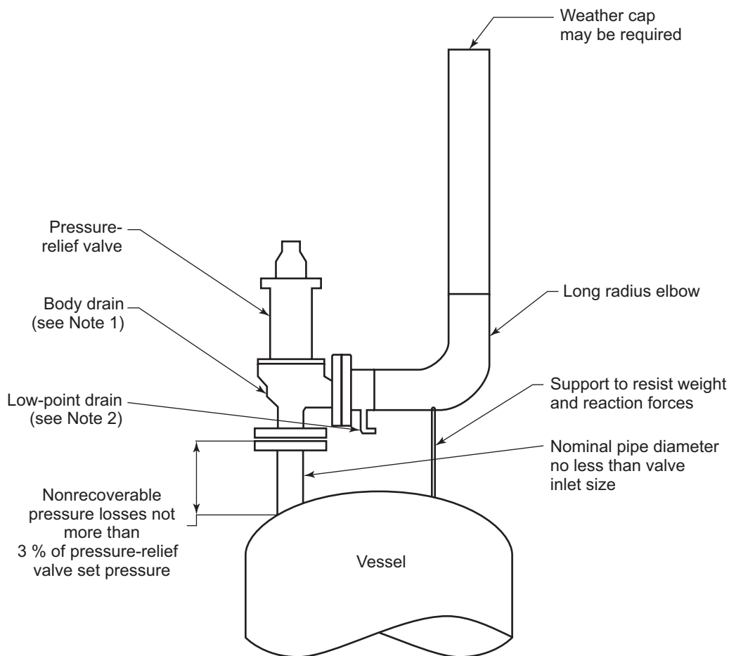
Figure 2—Typical Pressure-relief Valve Installation: Atmospheric (Open) Discharge
