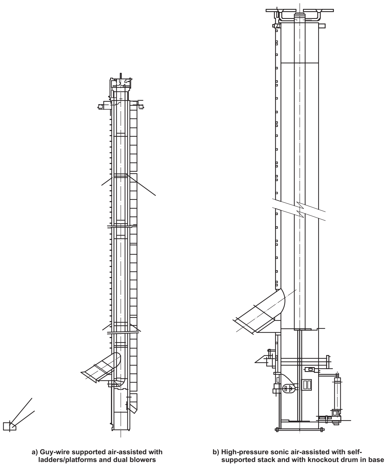
Figure 9—Typical Flare Systems
