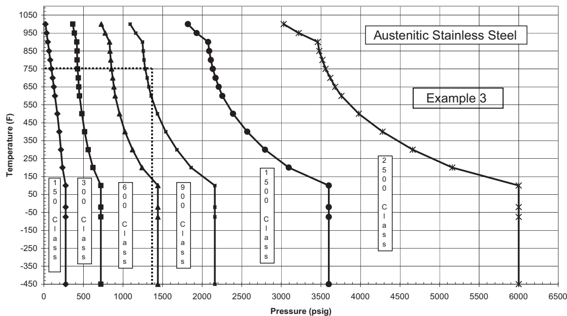
Figure D.2—Pressure-temperature Limits 1 for Example 3
