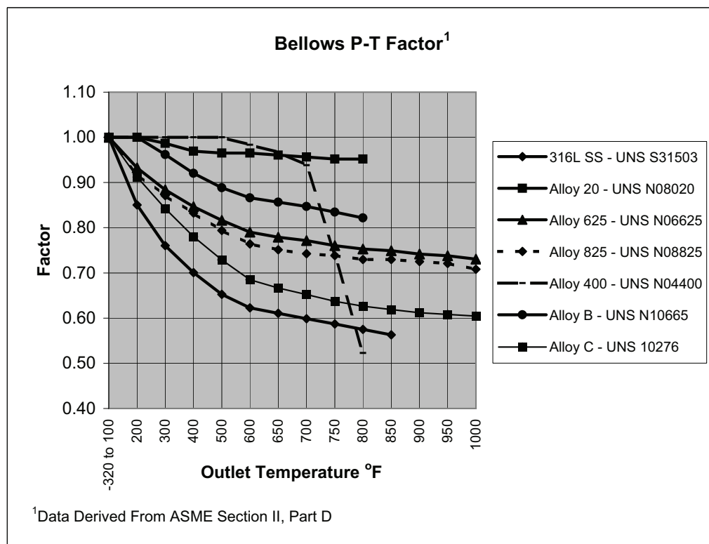
Figure C.1—Bellows Pressure-temperature Rating Factor
