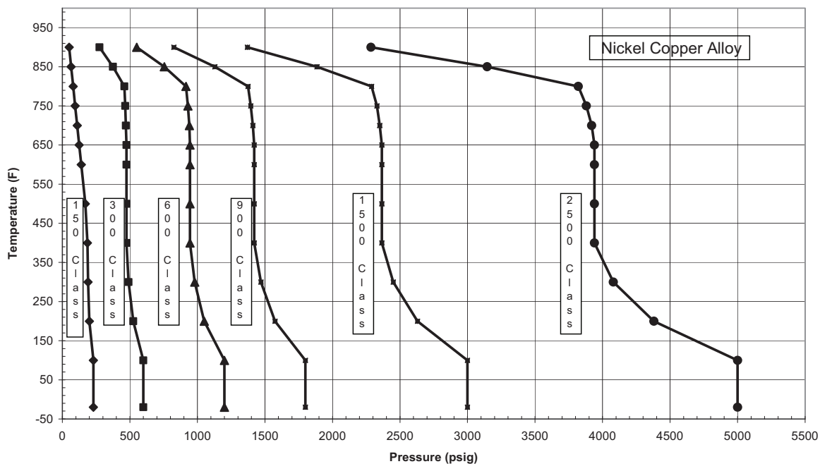
Figure B.4—Pressure-temperature Limits 1 to be Used with Table 3 to Table 30 of This Standard
