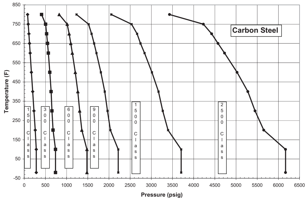
Figure B.1—Pressure-temperature Limits 1 to be Used with Table 3 to Table 30 of This Standard
