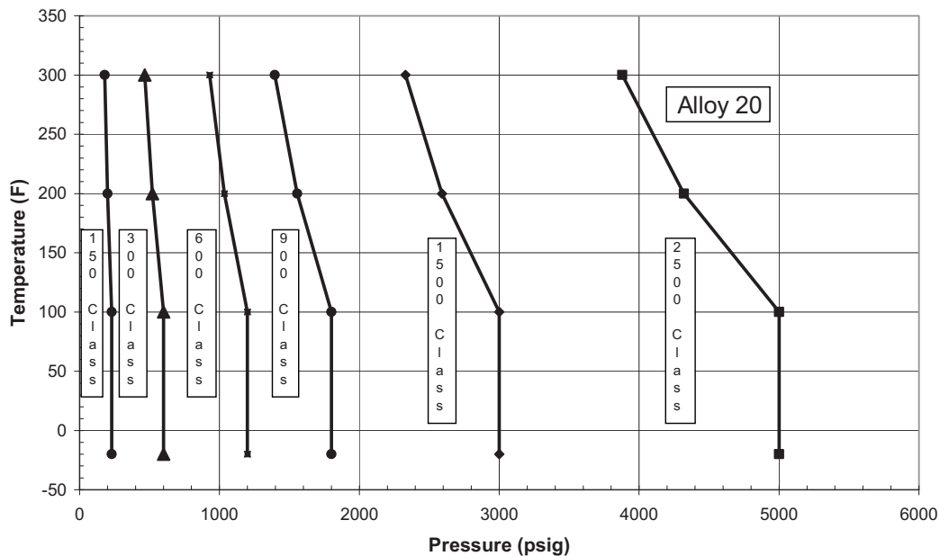
Figure B.5—Pressure-temperature Limits 1 to be Used with Table 3 to Table 30 of This Standard
