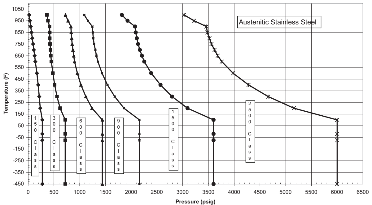
Figure B.3—Pressure-temperature Limits 1 to be Used with Table 3 to Table 30 of This Standard
