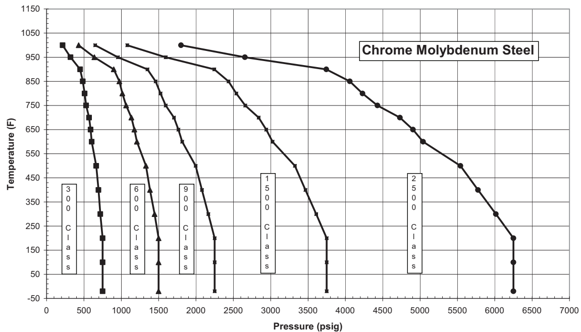
Figure B.2—Pressure-temperature Limits 1 to be Used with Table 3 to Table 30 of This Standard
