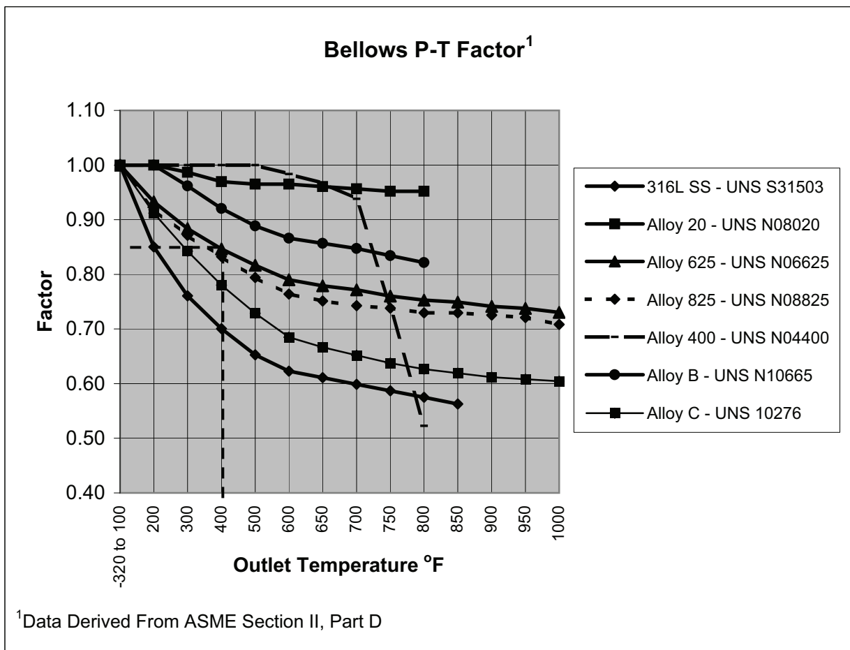
Figure D.1—Bellows Pressure-temperature Rating Factor for Example 2
