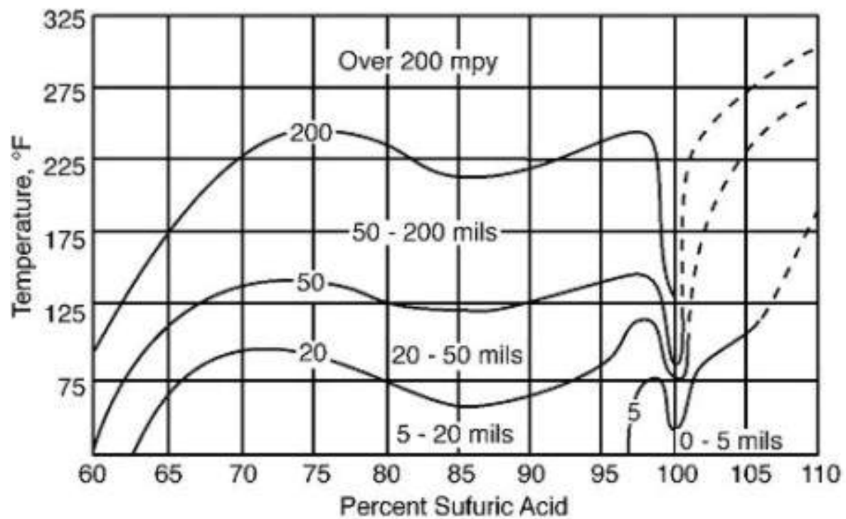
Figure 5-21 – Sulfuric acid corrosion data for carbon steel.
