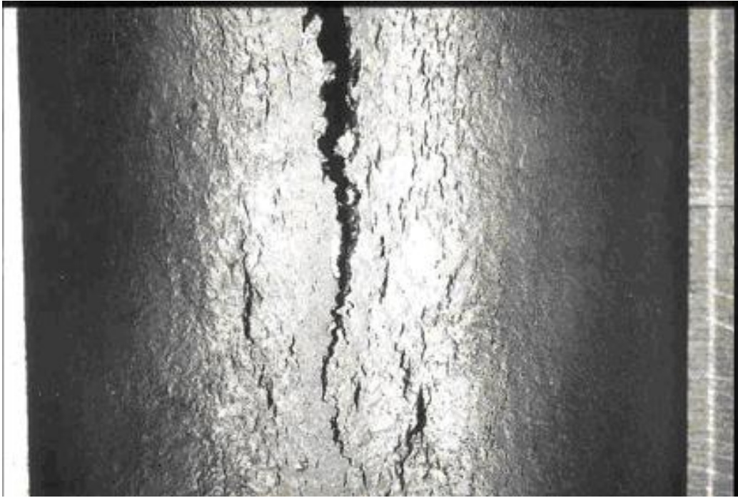
Figure 4-18 – Creep rupture of an HK40 heater tube.
