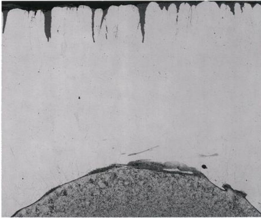
Figure 4-129 – On waterwall tubes, even with a corrosion-resistant weld-overly, circumferential cracking will develop. Mag. 37\frac{1}{2}X , etched.
