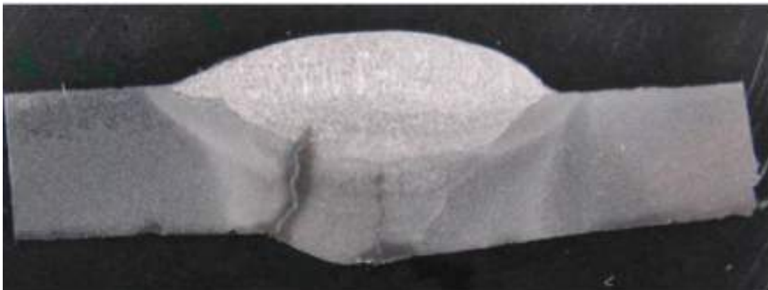
Figure 5-49 – Most cracks originate in base metal but this weldment contained a crack that originated at the root and propagated through the weld metal. Other cracks appear to have initiated in the HAZ (Reference 7).
