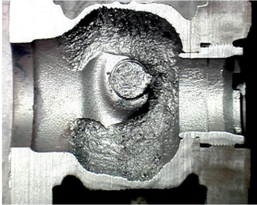
Figure 4-46 – Cutaway of a CS butterfly valve with cavitation damage after two years of service due to a high pressure drop across the valve in a hydrocarbon drain line off a cold low pressure separator in an atmospheric resid desulfurizing unit.
