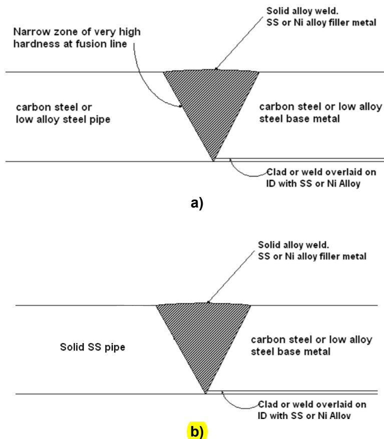
Figure 4-33 – Two primary DMW configurations.
