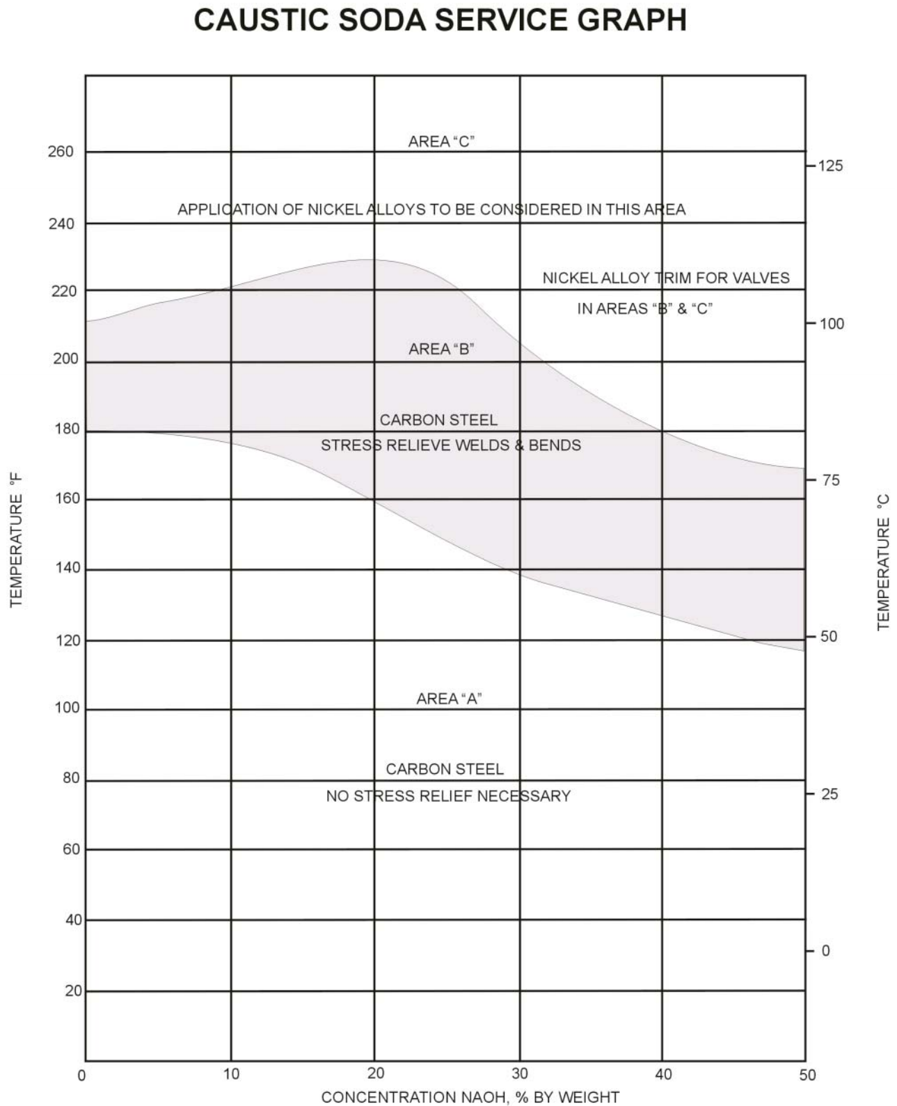
Figure 4-146 – Recommended operating limits for carbon steel in caustic service. (Reference 1)
