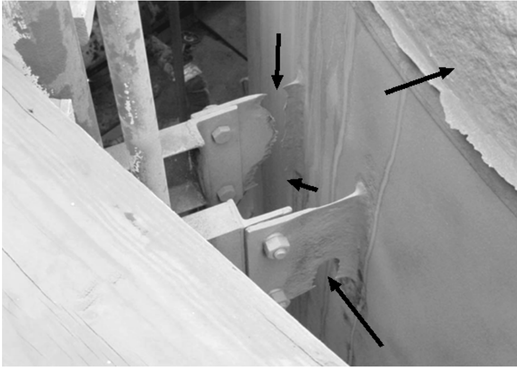
Figure 4-79 – CUI at attachment supports and vessel head.
