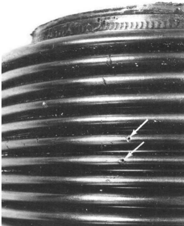
Figure 24—Pit-type Corrosion on 18Cr-8Ni Steel (Type 316) Bellows
