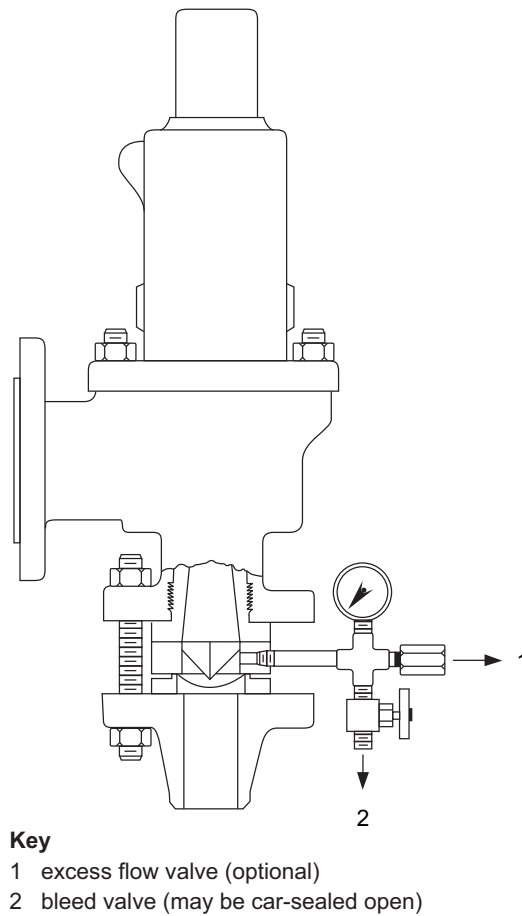
Figure 18—Combination of Reverse-buckling Disk Assembly and Safety-relief Valve
