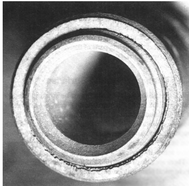
Figure 20—Acid Corrosion on 18Cr-8Ni Steel Inlet Nozzle
