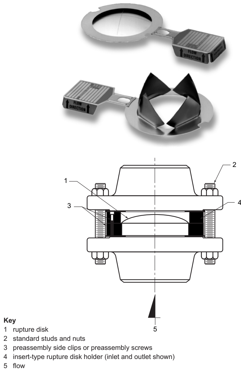
Figure 14—Scored Tension-loaded Rupture Disk
