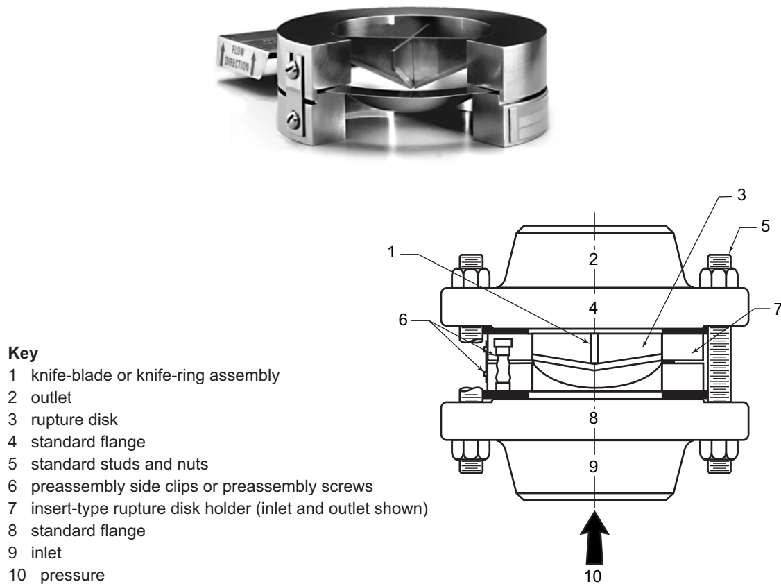
Figure 16—Reverse-acting Scored Rupture Disk with Knife Blades
