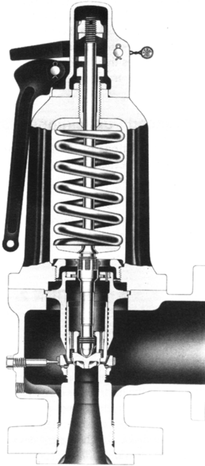
Figure 1—Full-nozzled, Top-guided Safety Valve
