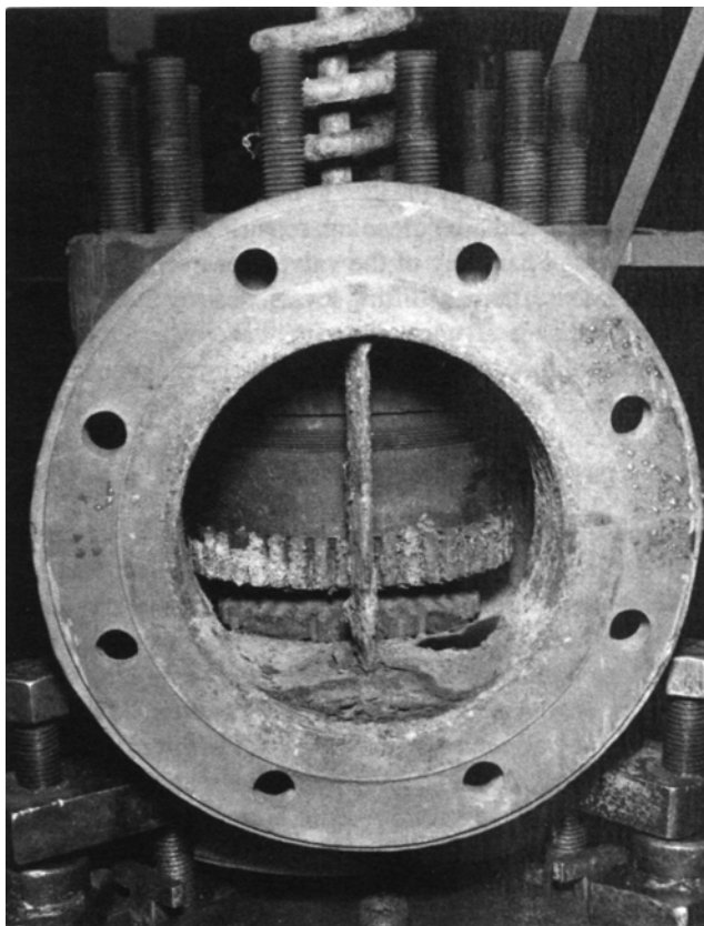
Figure 34—Spring Failure Due to Stress Corrosion
