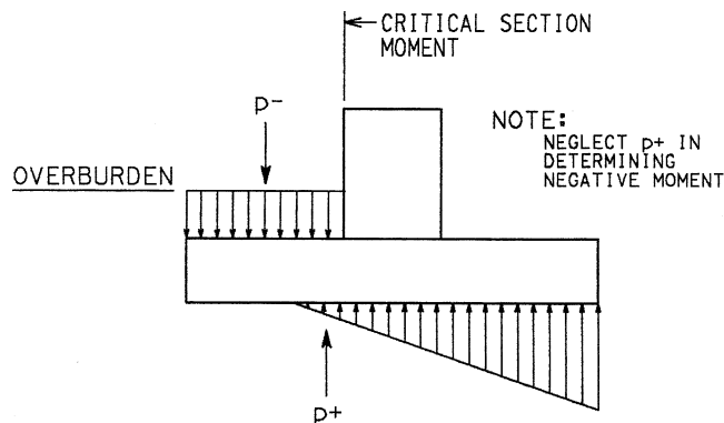
Fig. 5.9—Negative moment.
