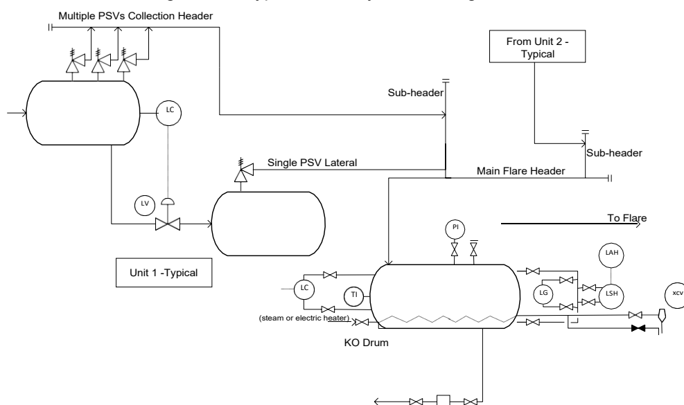
Figure 8.1. Typical Flare System Arrangement
