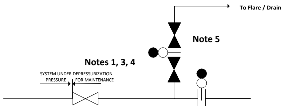
Figure 9.1- Single Block & Bleed Isolation
