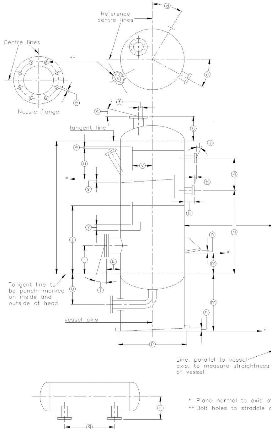
Figure 1: Tolerances - Alphabetic coding
