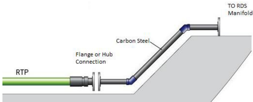
Fig. 4 – RTP Approach Connectivity (Outside the Fence)
