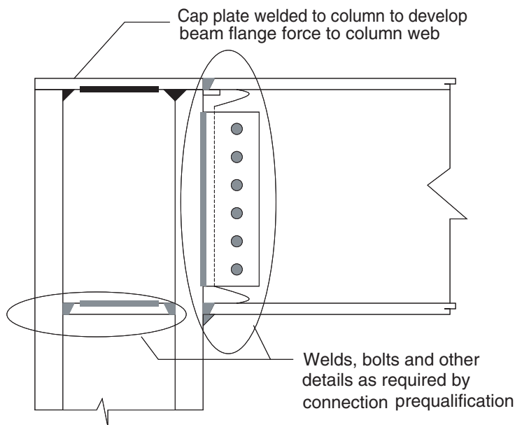
Fig. C-2.2. Cap plate detail at column top.
