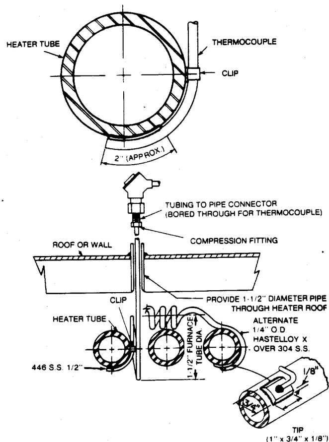
Figure 3-11—Heater Tube Skin Thermocouple Installation
