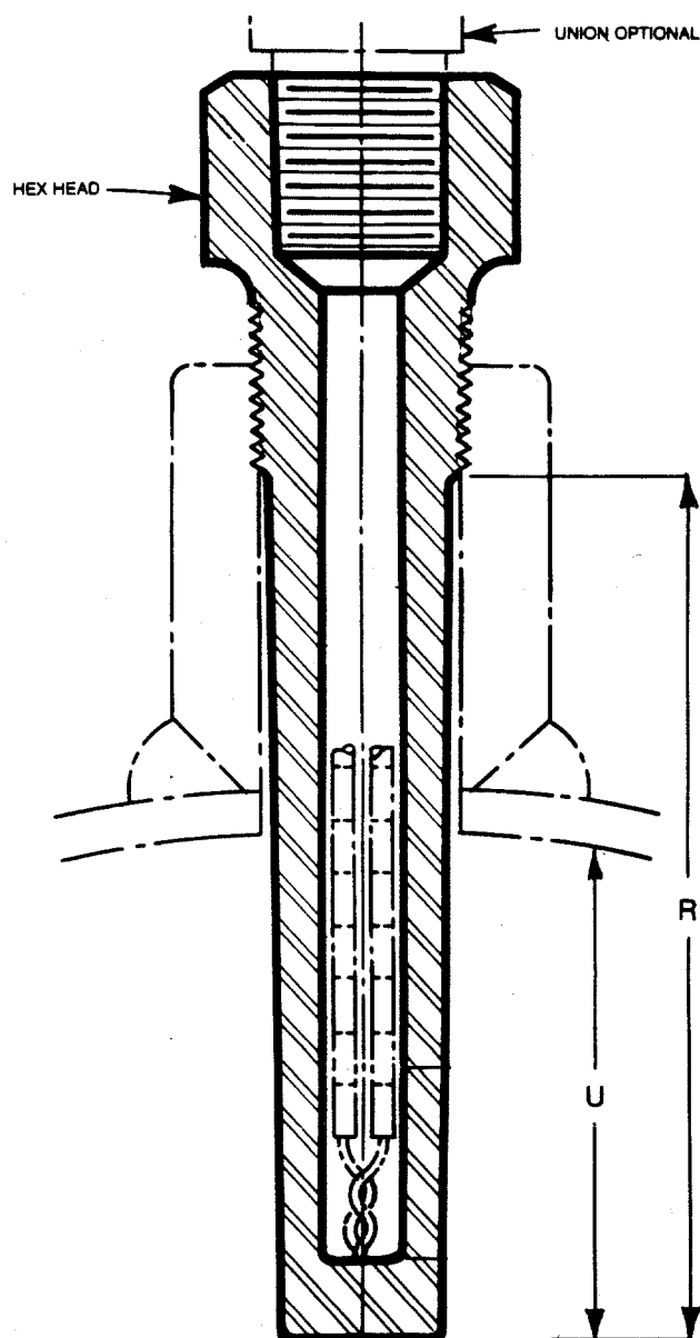
Figure 3-1—Screwed Thermowell
