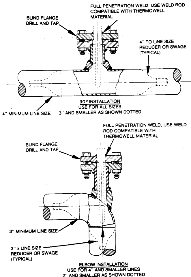
Figure 3-6—Typical Flanged Thermowell Installation
