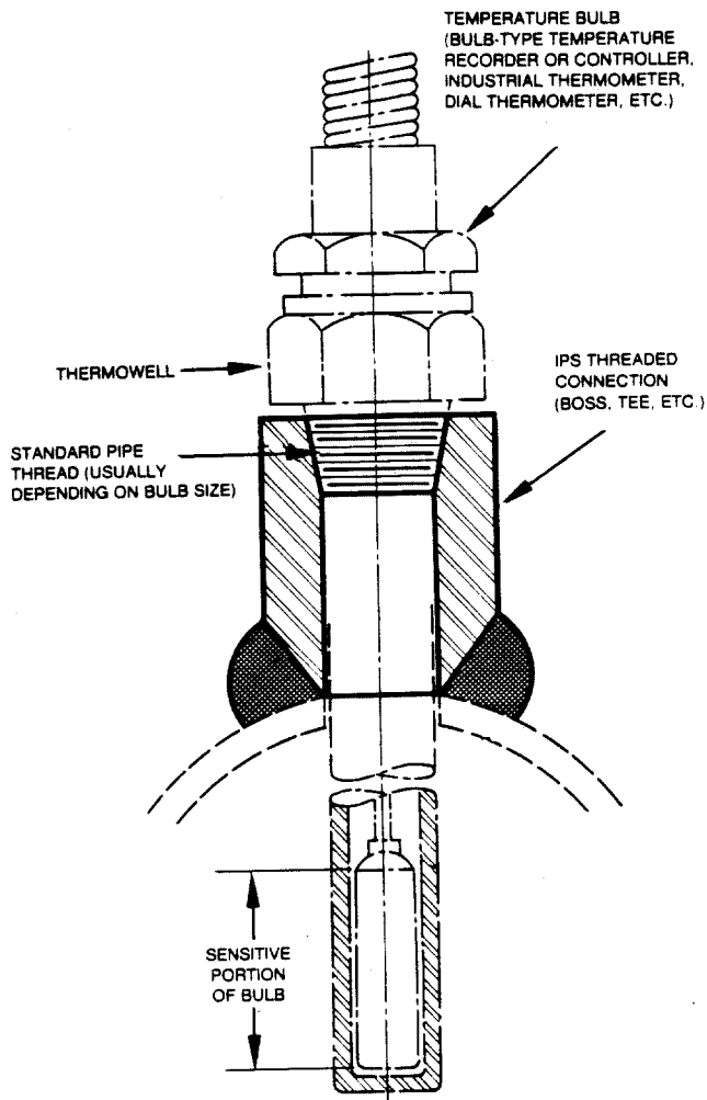
Figure 3-4—Temperature Bulb Installation
