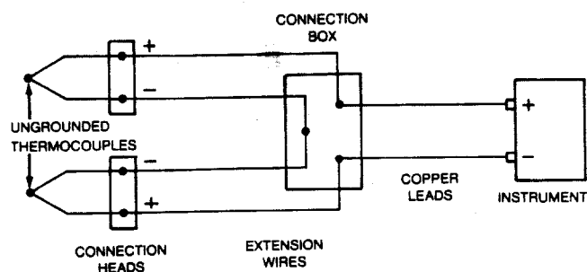
Figure 3-14—Temperature Difference Measurement With Thermocouples
