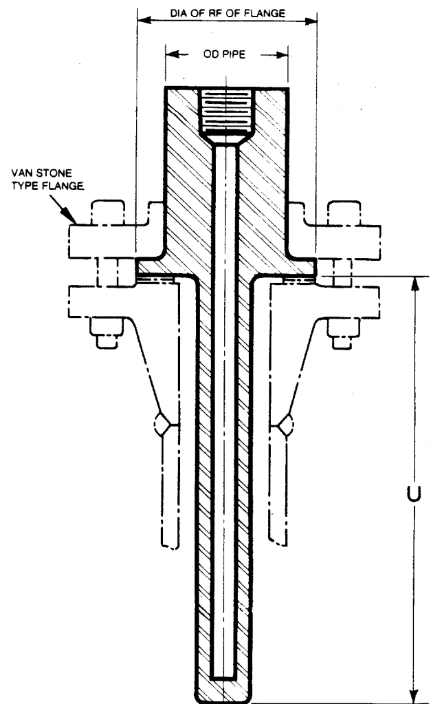
Figure 3-3—Flanged Thermowell—Van Stone
