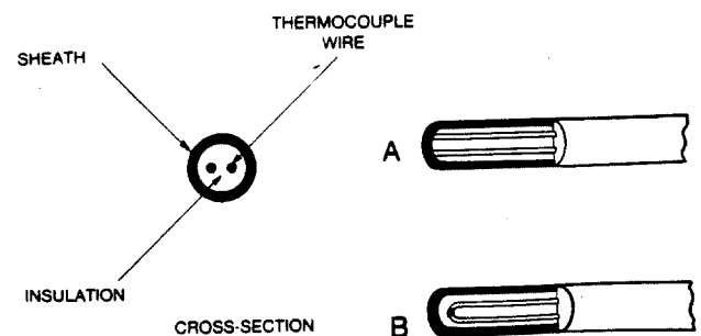
Figure 3-7—Metal-Sheathed, Mineral-Insulated Thermocouple Assemblies
