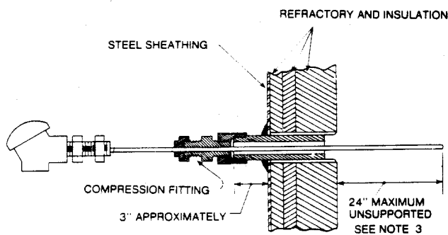
Figure 3-12—Typical Firebox Thermocouple Installations
