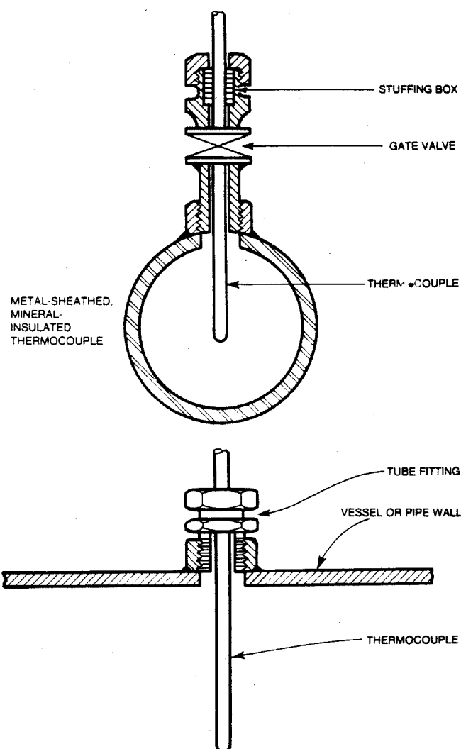
Figure 3-9—Installation of Thermocouples Without Wells
