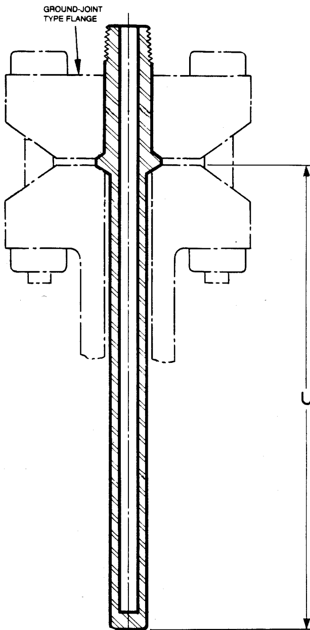
Figure 3-2—Ground-Joint Thermowell
