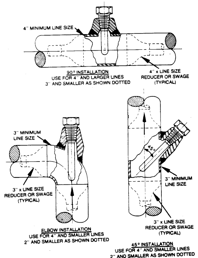
Figure 3-5—Typical Screwed Thermowell Installation
