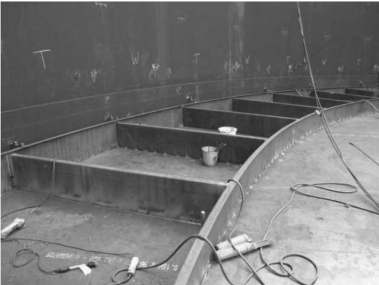
Pontoon construction.
