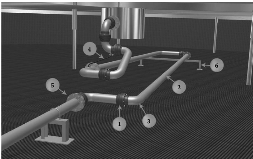
Swivel joint articulated drain system.
