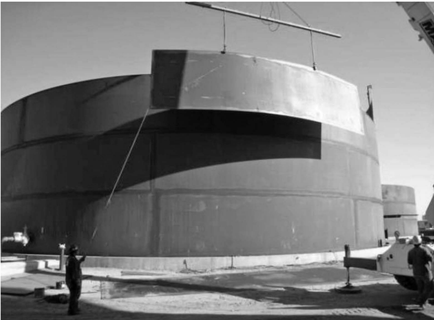
Fourth shell course erection in progress (view from outside).
