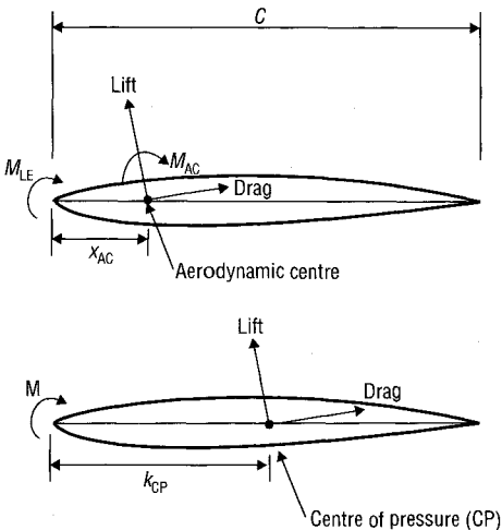
Fig. 6.5 Aerodynamic centre and centre of pressure
