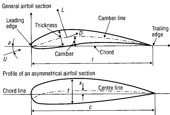
Fig. 6.2 Airfoil sections: general layout
