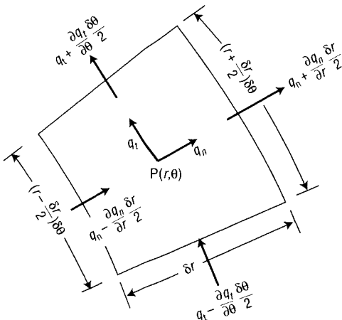
Fig. 5.3 The continuity equation basis in 2-D
