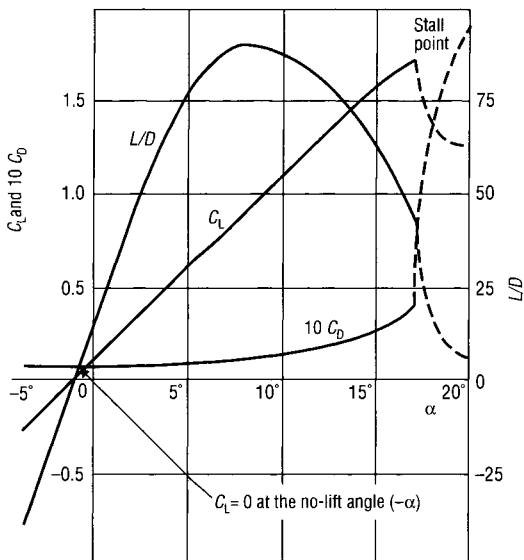
Characteristics for an asymmetrical 'infinite-span 2D airfoil'
