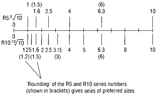
Fig. 12.2 The R5 and R10 series
