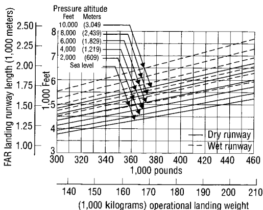
Fig. 11.11 Aircraft:airport compatibility – landing runway length requirements. Figure shows Boeing 777-200. Courtesy Boeing Commercial Airplane Group
