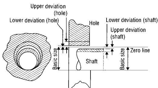
Fig. 12.8 Principles of a shaft-hole fit
