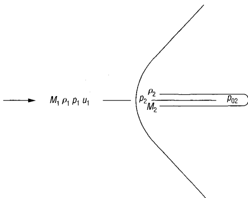
Fig. 5.11 Pitot tube relations
