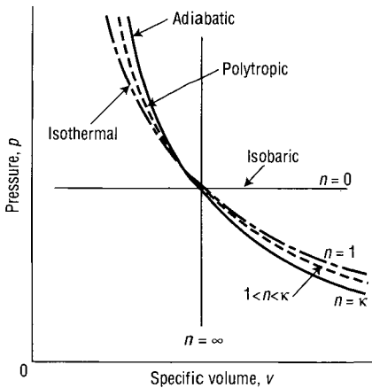
Fig. 5.1 Changes of state of a perfect gas
