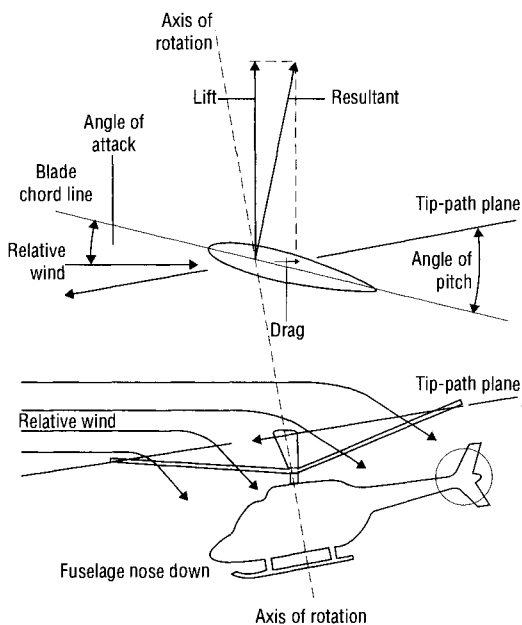
Fig. 10.6 Helicopter principles: lift and propulsion
