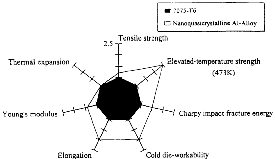
Figure 11.14. Property envelope for nanoquasicrystalline alloy, compared with 7075.
