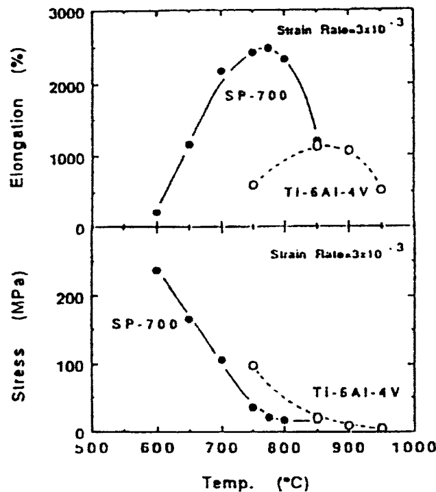
Figure 2.8. Superplastic elongation and flow stress of SP700.
