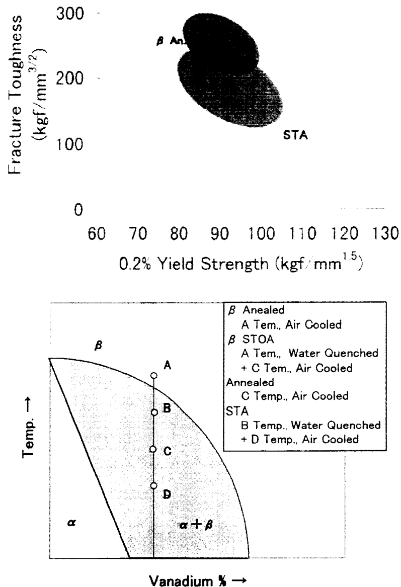
Figure 2.6. Mechanical properties of \alpha + \beta Ti-6Al-4V heat treated under different conditions.
