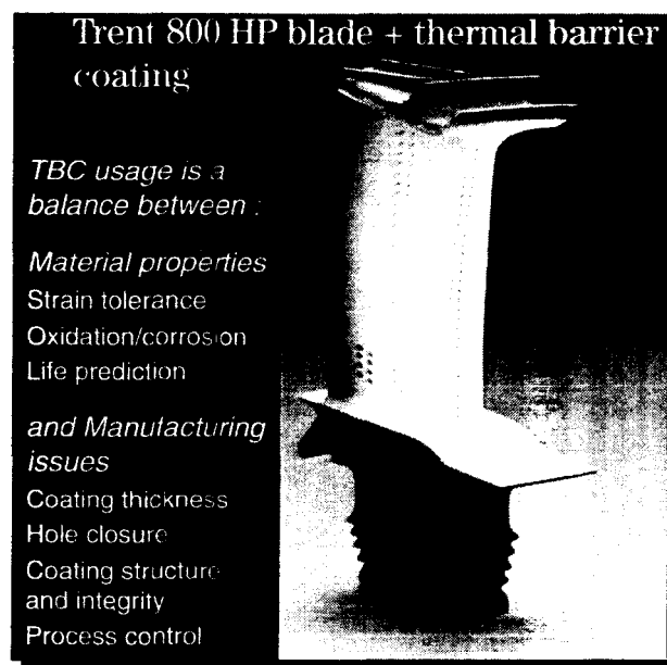
Figure 7.5. Trent 800 high pressure (HP) turbine blade, showing cooling holes and thermal barrier coating (TBC).
