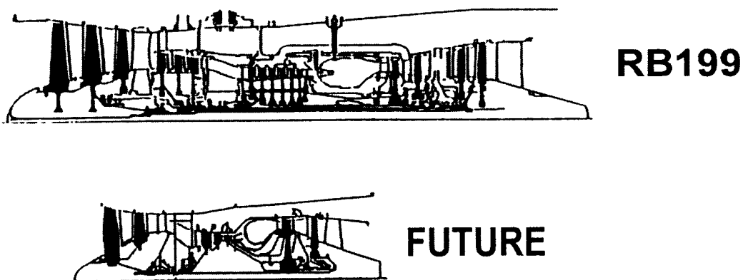
Figure 9.4. Targets for future military engines include increased thrust to weight ratios and reduced engine cross sections (after Ruffles [3]).
