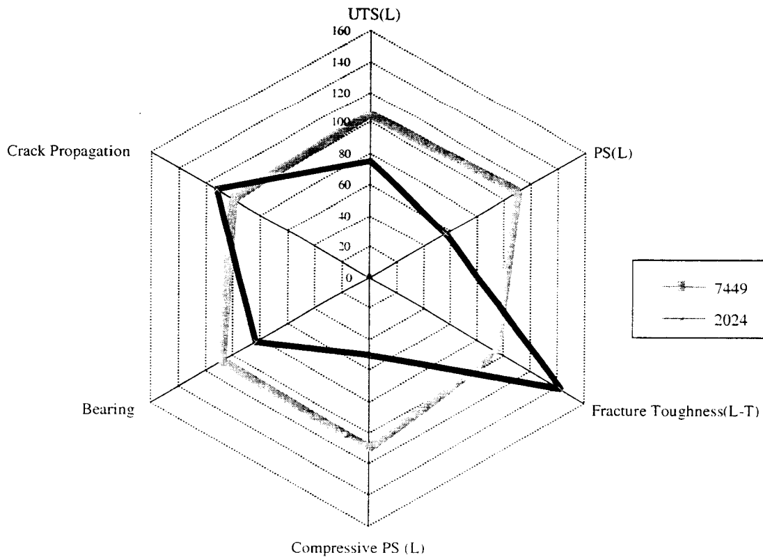
Figure 1.8. Property envelopes for aluminium alloys 7449 and 2024.
