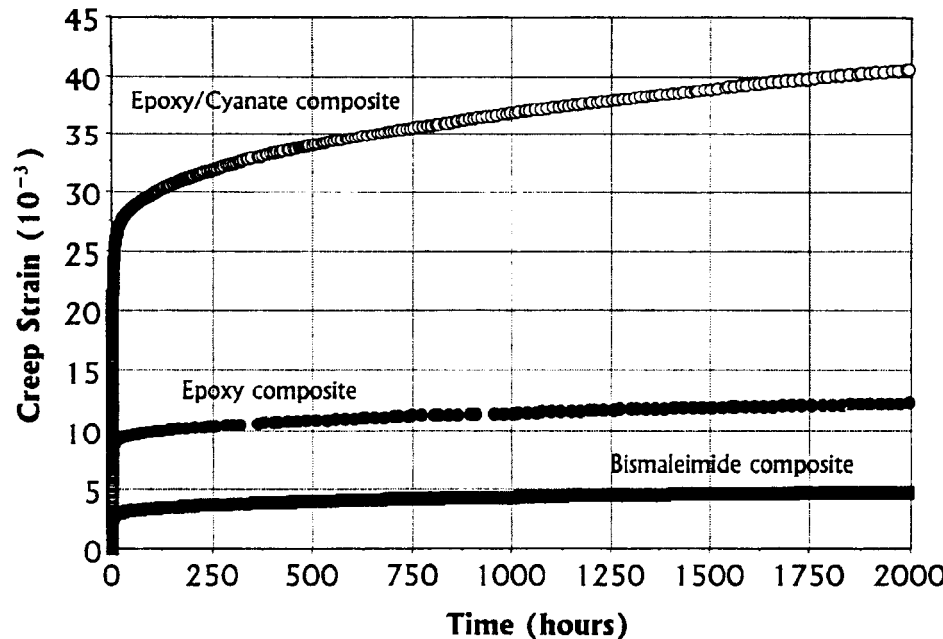
Figure 3.7. Creep testing on [\pm 45^\circ]_{4S} laminates at 120°C, 70 MPa.
