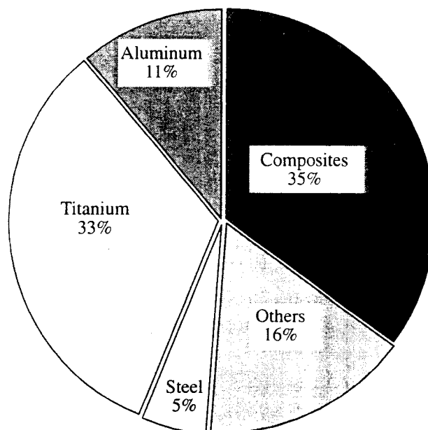
Figure 2.5. Material distribution on the F-22 fighter.
