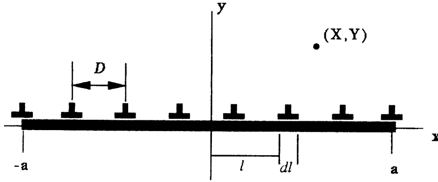
Figure 20.10. Calculation of stresses generated by an array of edge dislocations on the \gamma/\gamma' interface.
