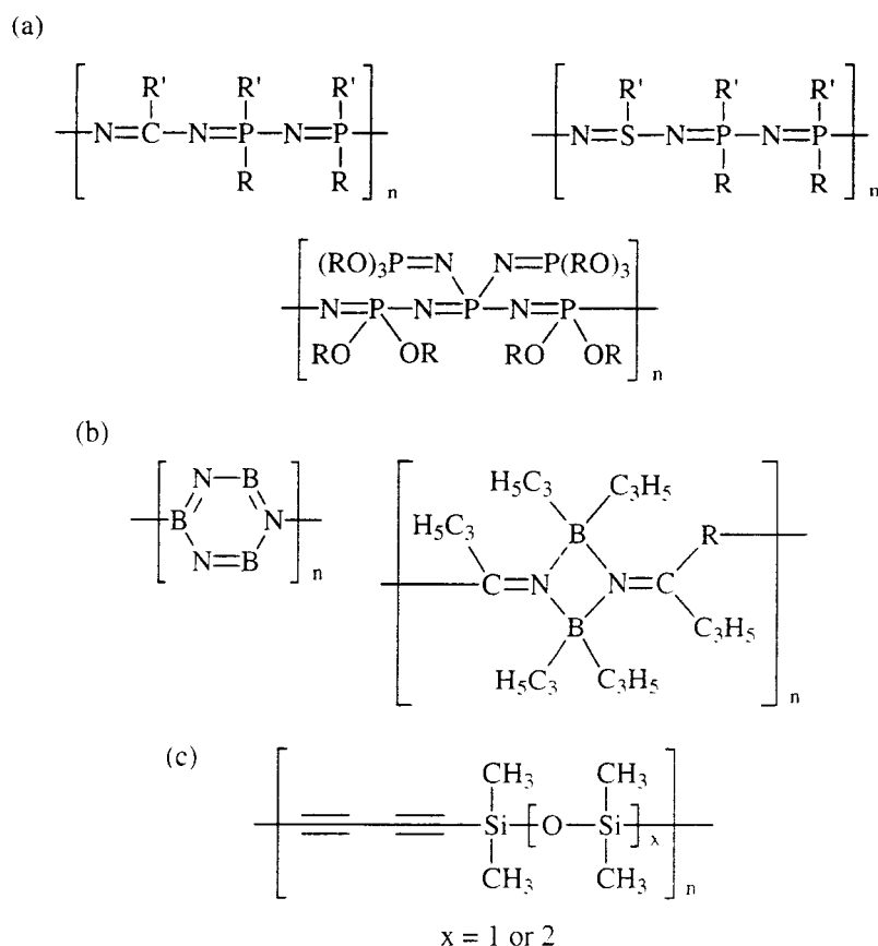
Figure 13.3. Potential polymers for use in ultra-high temperature matrix systems: (a) modified polyphosphazenes (b) boron-based compounds and (c) siloxane-acetylene.
