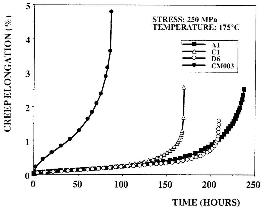
Figure 3.1. Creep curves at 175°C/250 MPa.
