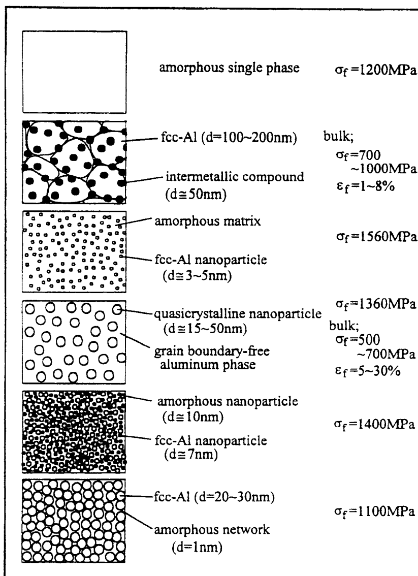
Figure 11.1. Schematic nonequilibrium alloy structures.
