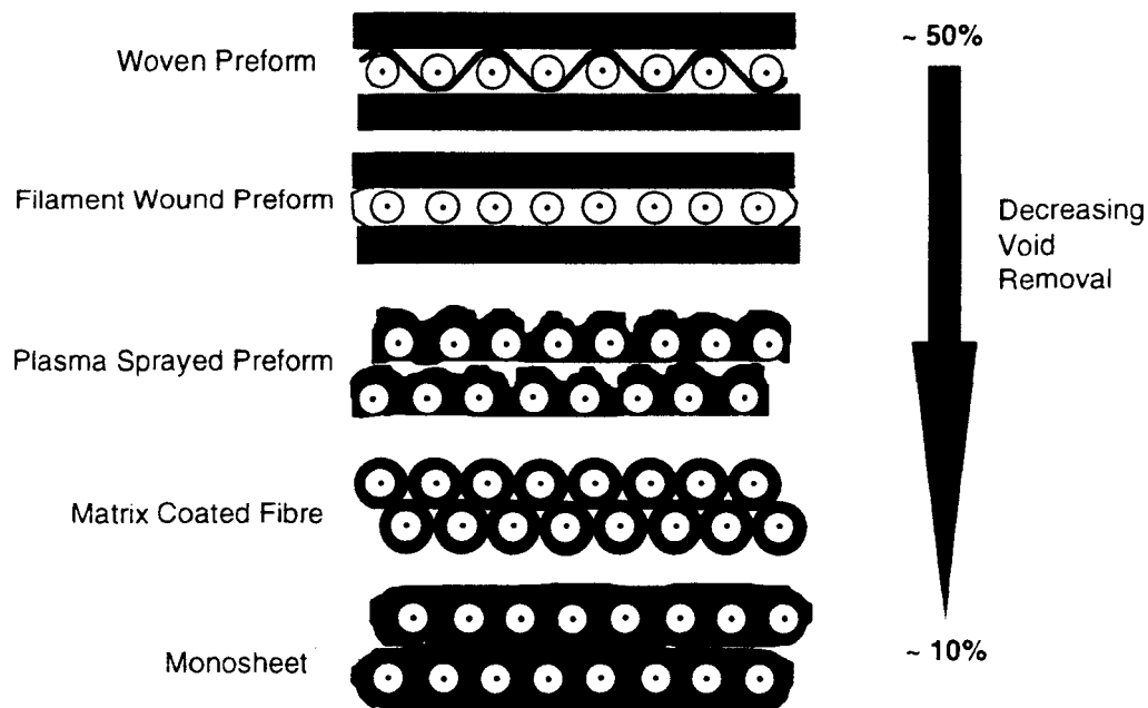
Figure 18.8. Debulking associated with different titanium MMC processing methods.
