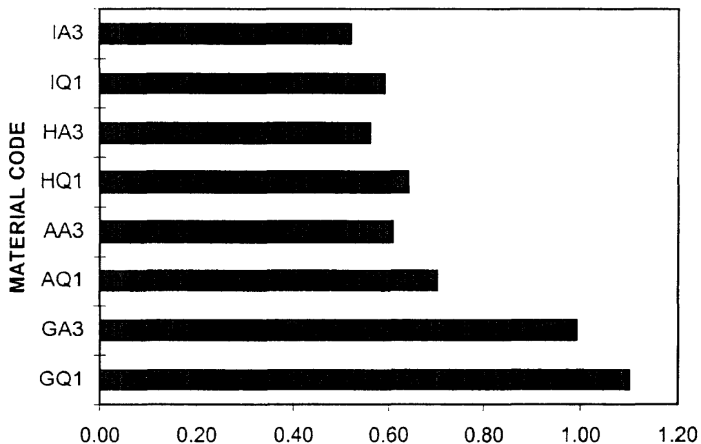
Figure 16.1. Mass for equal bending stiffness—normalized to aluminium alloy 2024.
