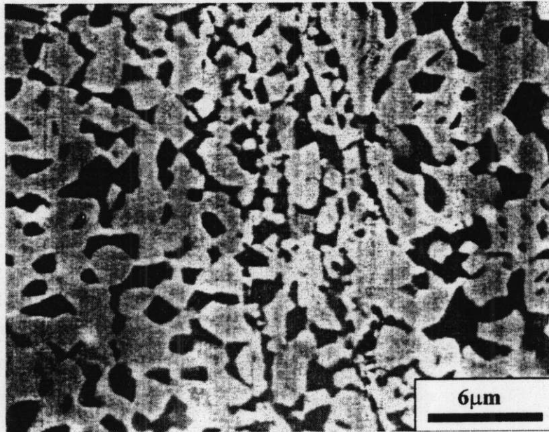
Figure 22.4. SEM micrograph of typical CoNiCrAlY \gamma/\beta microstructure after heat treatment.
