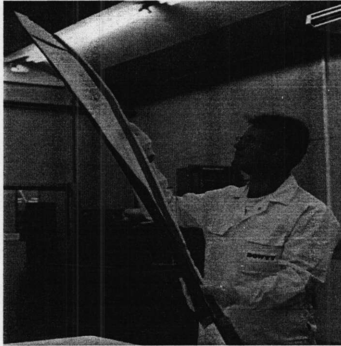
Figure 6.5. Blade preform.
