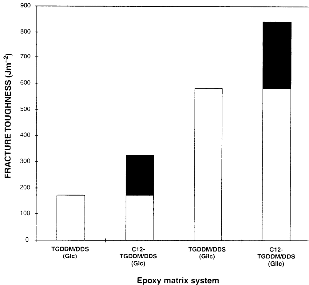
Figure 15.7. Comparison of fracture energies G_{IC} and G_{IIC} of the proprietary TGDDM and Cl_2 -TGDDM composite systems at 20 °C (post-cured at 180 °C).
