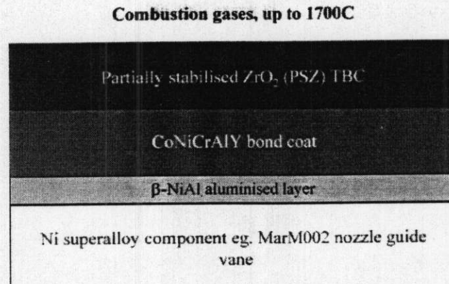
Figure 22.1. Schematic of a typical TBC arrangement.
