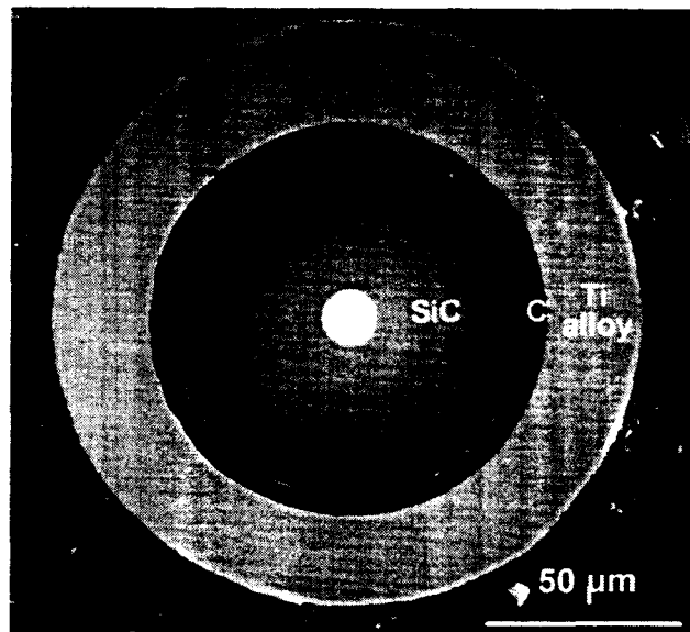
Figure 18.3. A matrix coated silicon carbide fibre.
