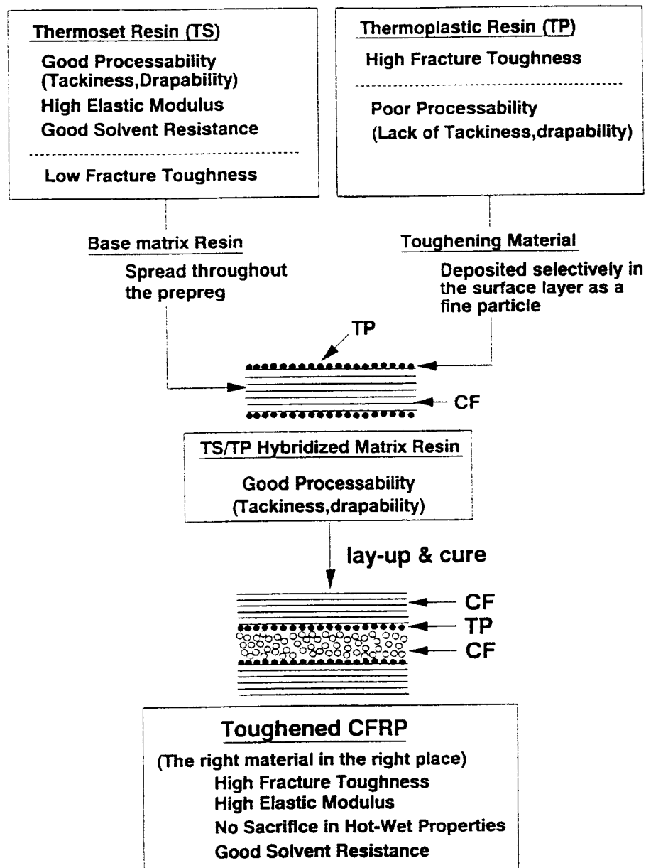
Figure 14.8. Concept of thermoplastic-particulate interlayer toughened pre-preg.
