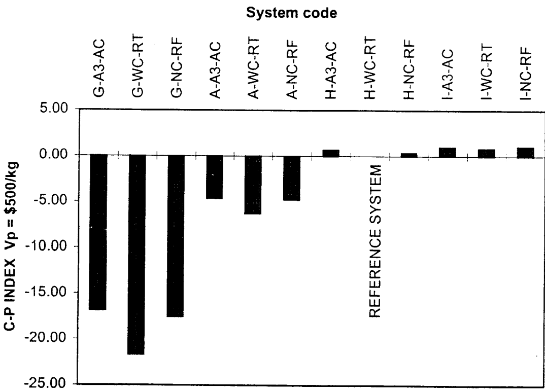
Figure 16.5. Cost performance indices ( v_p = 500 \$/\text{kg}^{-1} ).
