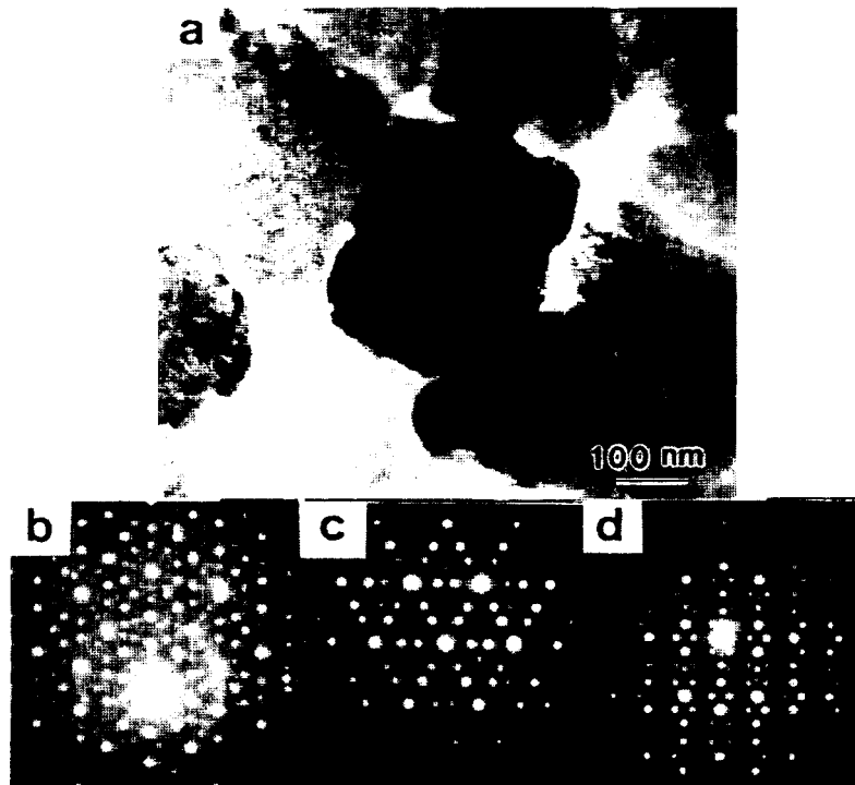
Figure 11.12. Structure and diffraction patterns from icosahedral Al-Fe-Cr-Ti.
