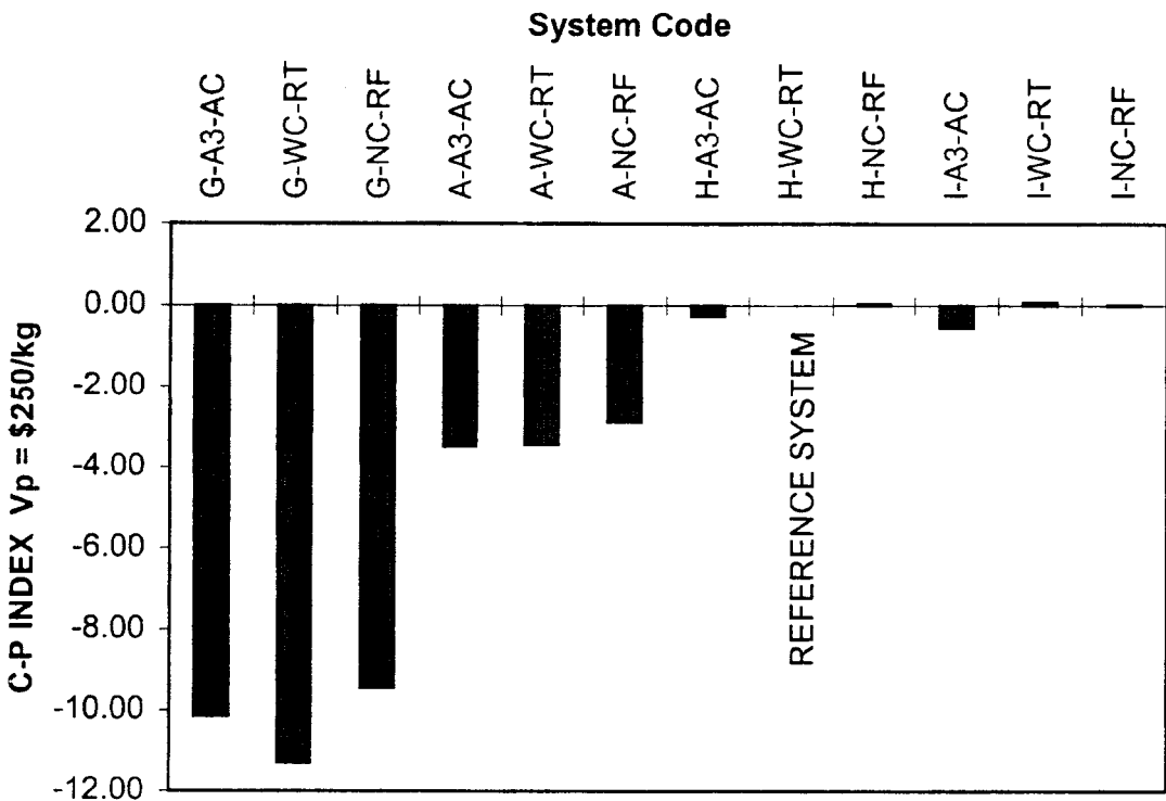
Figure 16.4. Cost performance indices ( v_p = 250 \$/\text{kg}^{-1} ).
