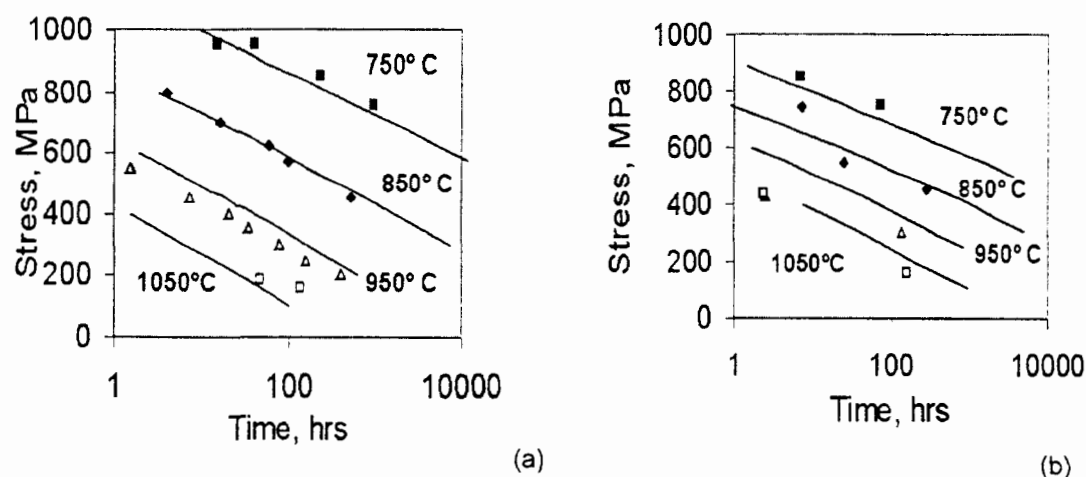
Figure 19.3. Comparison of model predictions and creep data of times to achieve arbitrary creep strains in SRR99 at various temperatures and stresses (a) \langle 001 \rangle , time to 5% strain, and (b) \langle 111 \rangle , time to 2% strain.
