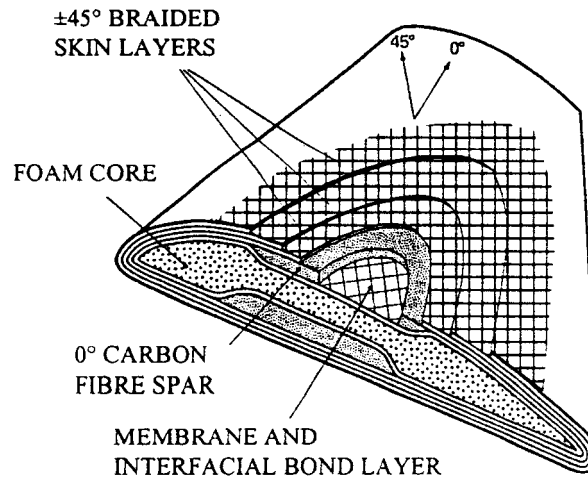
Figure 6.4. Blade root construction.
