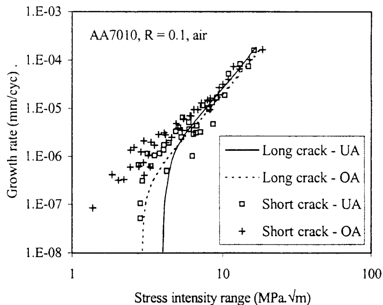
Figure 10.6. Heat treatment effect on short crack growth rates (after Bolingbroke and King [54]).
