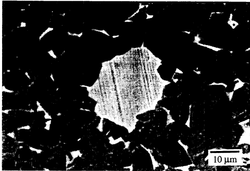
Figure 17.1. Scanning electron micrograph of a HIPed sample of atomized Ti-48Al-2Mn-2Nb showing a region with a lamellar structure, despite the fact that the sample was HIPed well below the \alpha transus. EDX shows this region to be relatively rich in Ti.
