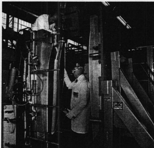
Figure 6.8. Preform and resin transfer mould.
