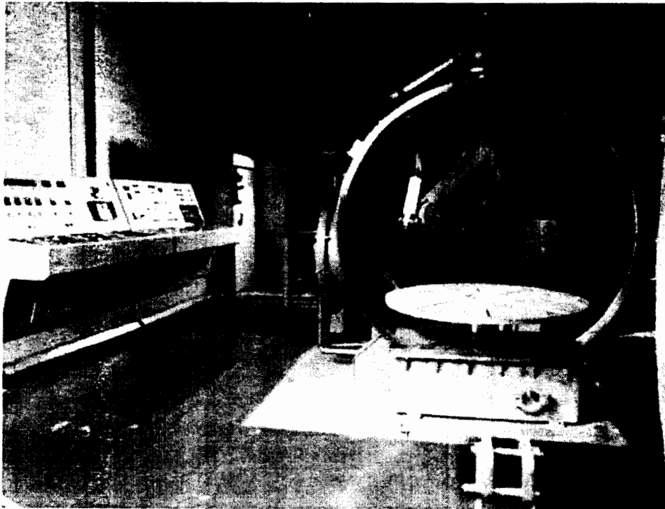
Figure 22.10. A VPS system for the manufacture of MCrAlY coatings.
