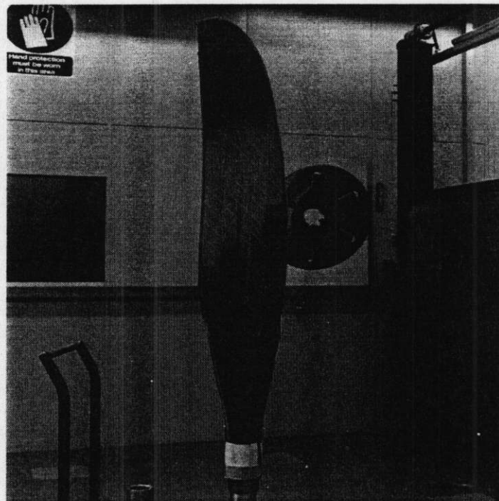
Figure 6.6. Preform after foam injection.
