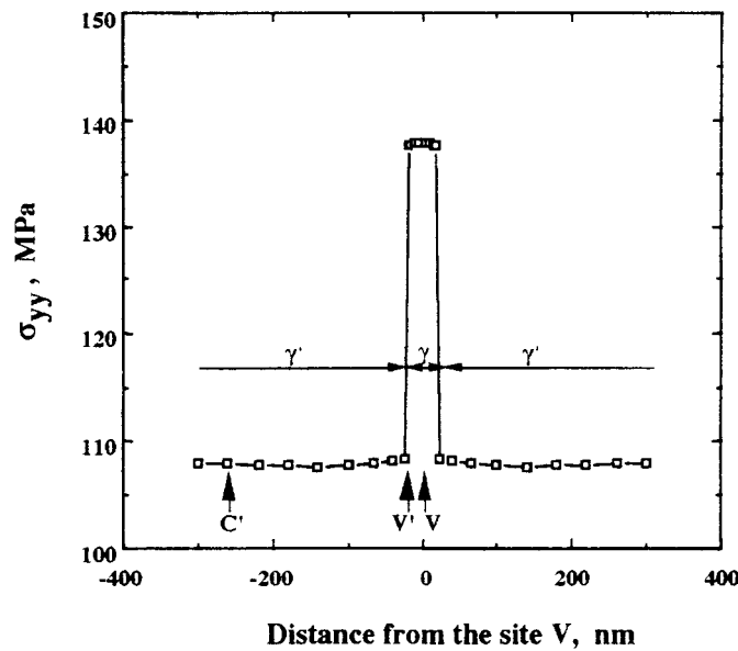
Figure 20.5. Finite element analysis of the stress distribution due to an external force. The elastic constants obtained for f = 0 are used and the average stress, \sigma , in the loading direction is 110\text{ MPa} .
