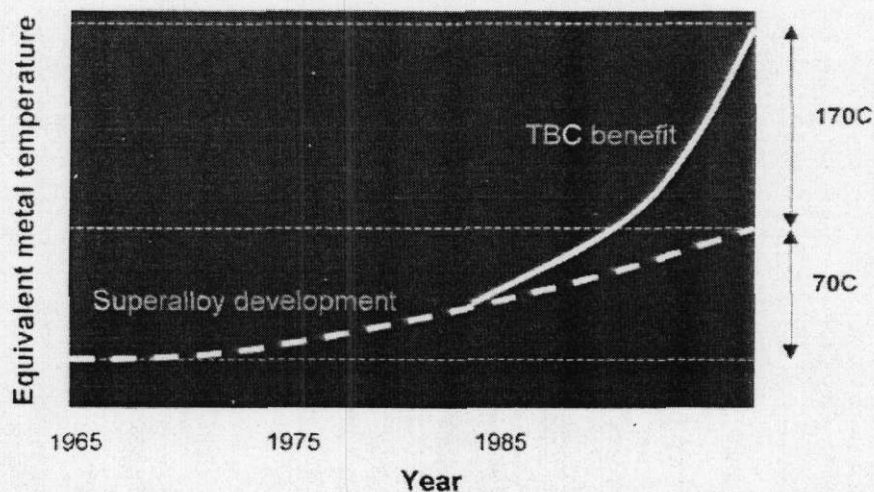
Figure 22.2. Operating temperature advantage offered by TBCs [1].
