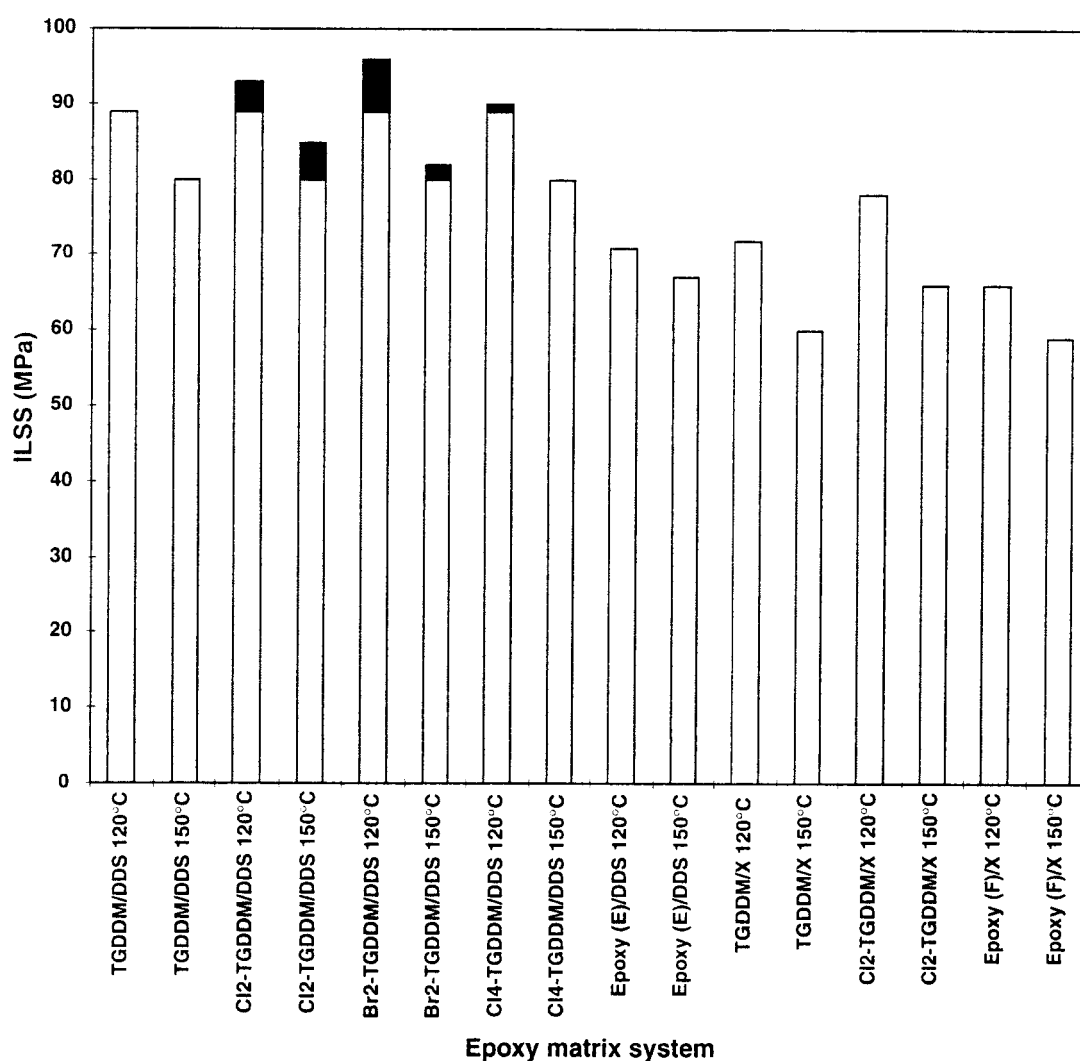
Figure 15.3. Mean interlaminar shear strength (MPa) of unaged composites tested at 120°C and 150°C.
