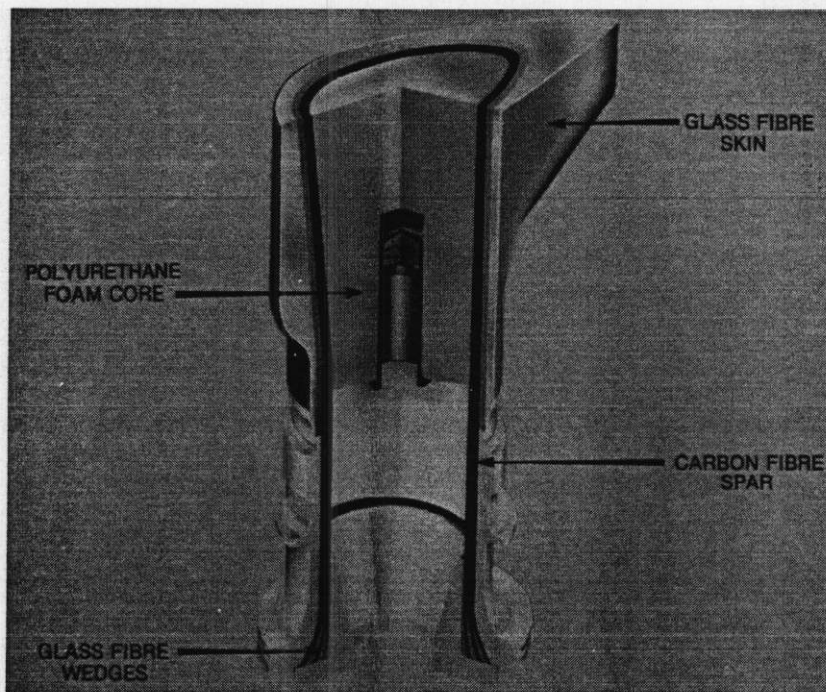
Figure 6.3. Composite blade construction.
