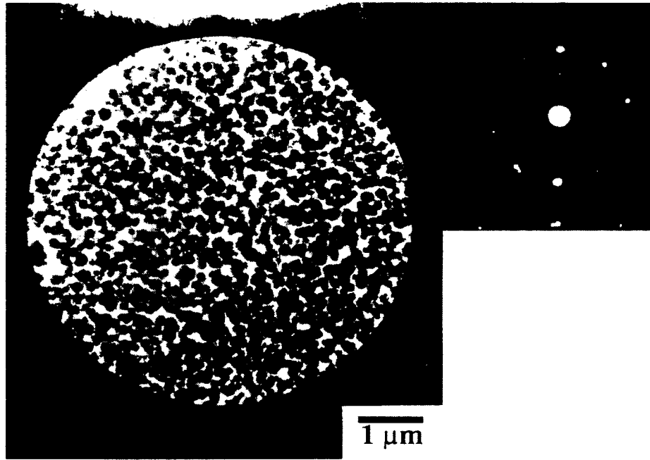
Figure 11.9. Structure of icosahedral Al-Mn-Co alloy.
