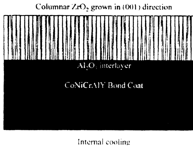
Figure 22.12. Schematic of a typical EB-PVD processed TBC microstructure.
