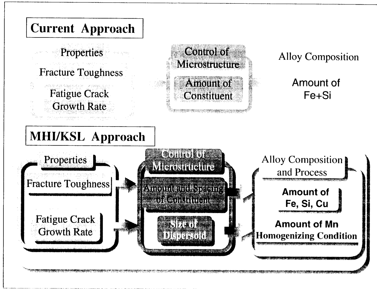
Figure 2.1. New approach to improving fracture toughness and fatigue crack growth rate.
