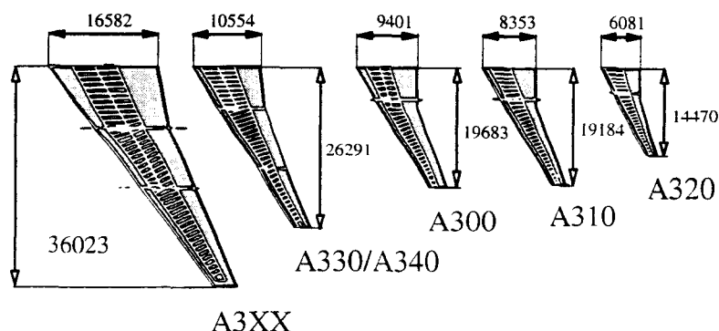
Figure 1.2. Wing sizes for modern large body aircraft.
