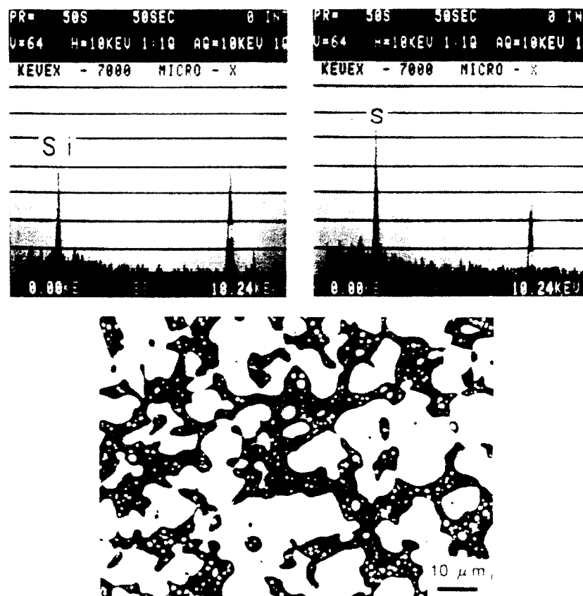
Figure 14.3. Scanning electron micrograph (backscattered electron mode) of epoxy, PI-Si cured resin: (1) darker phase: imide oligomer-rich phase which contains silicon, (2) brighter phase: epoxy-rich phase which contains sulphur.
