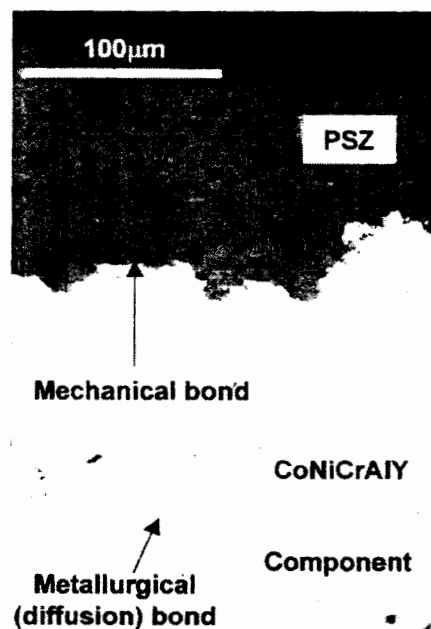
Figure 22.11. A typical plasma sprayed TBC arrangement.
