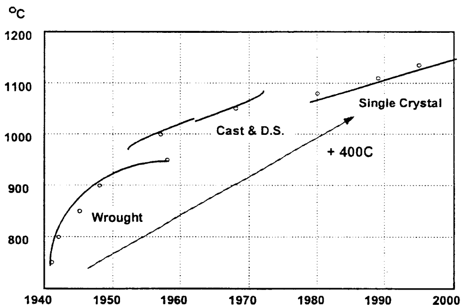
Figure 7.4. Temperature capability of different turbine blades since 1940.
