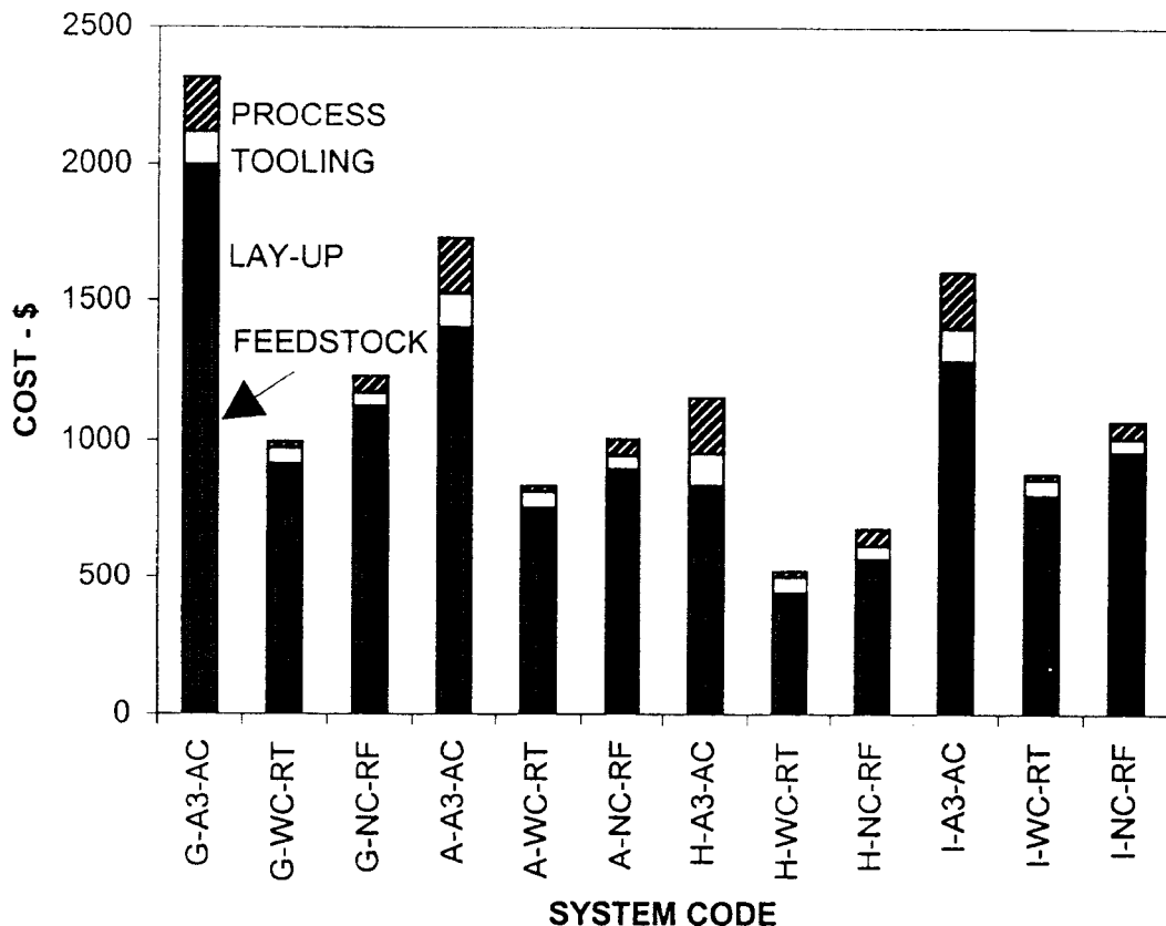
Figure 16.3. Cost for equal in-plane stiffness.
