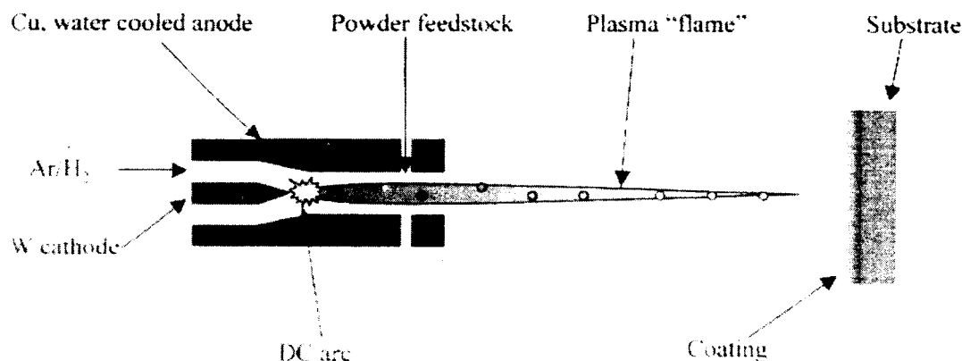
Figure 22.9. A schematic of plasma spraying.
